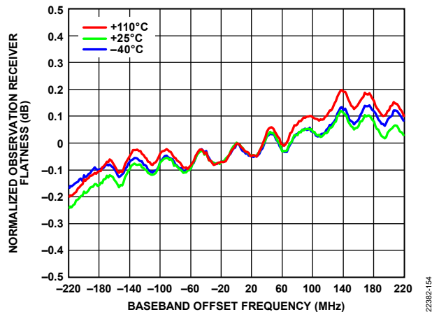
Figure 225. Normalized Observation Receiver Flatness vs. Baseband Offset Frequency, -10 dBFS Input Signal
