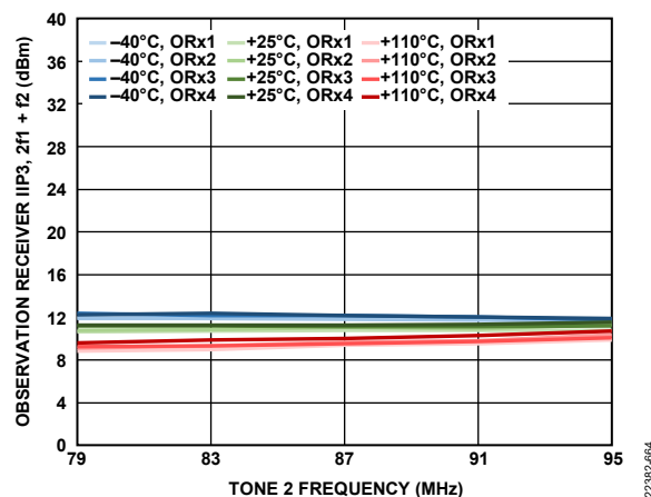
Figure 66. Observation Receiver IIP3, 2f_1 + f_2 vs. Tone 2 Frequency, Both Tones at -13 dBFS, f_1 = f_2 + 2 MHz
