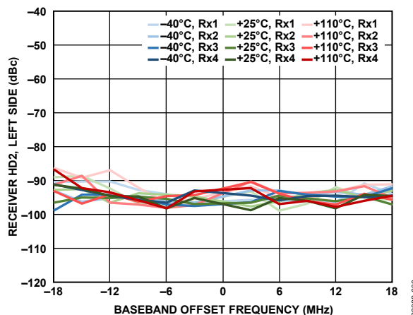
Figure 32. Receiver HD2, Left Side vs. Baseband Offset Frequency, -5 dBFS Input Signal, Distortion Tone Measured Left of 0 Hz (HD2 Canceller Enabled)
