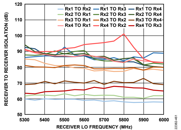
Figure 532. Receiver to Receiver Isolation vs. Receiver LO Frequency
