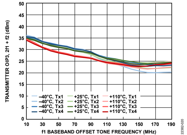
Figure 91. Transmitter OIP3, 2f_1 + f_2 vs. f_1 Baseband Offset Tone Frequency, f_2 = f_1 + 5 MHz, 15 dB Digital Back Off per Tone
