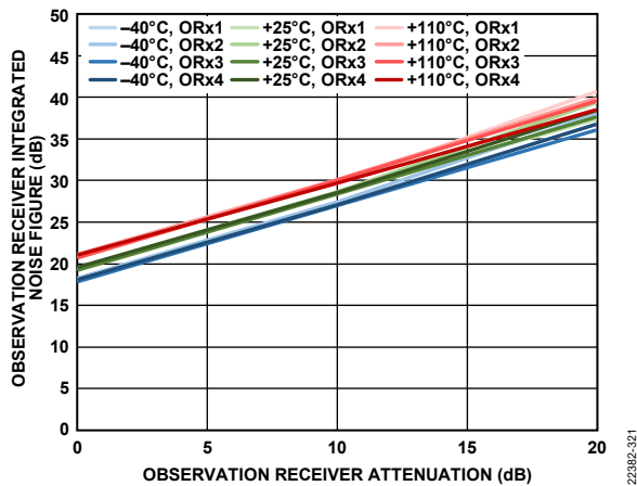
Figure 392. Observation Receiver Integrated Noise Figure vs. Observation Receiver Attenuation, 450 MHz Bandwidth, Sample Rate = 491.52 MSPS, Integration Bandwidth = 500 kHz to 245.76 MHz
