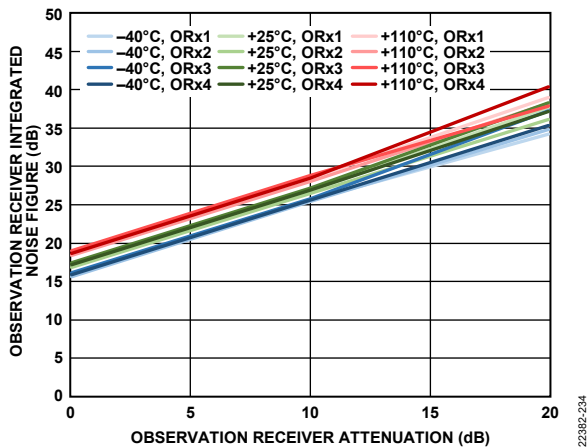
Figure 305. Observation Receiver Integrated Noise Figure vs. Observation Receiver Attenuation, 450 MHz Bandwidth, Sample Rate = 491.52 MSPS, Integration Bandwidth = 500 kHz to 245.76 MHz
