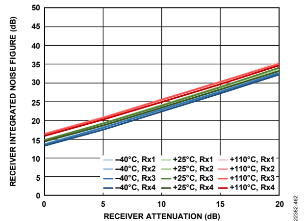
Figure 533. Receiver Integrated Noise Figure vs. Receiver Attenuation, 200 MHz Bandwidth, Sample Rate = 245.76 MSPS, Integration Bandwidth = 500 kHz to 100 MHz
