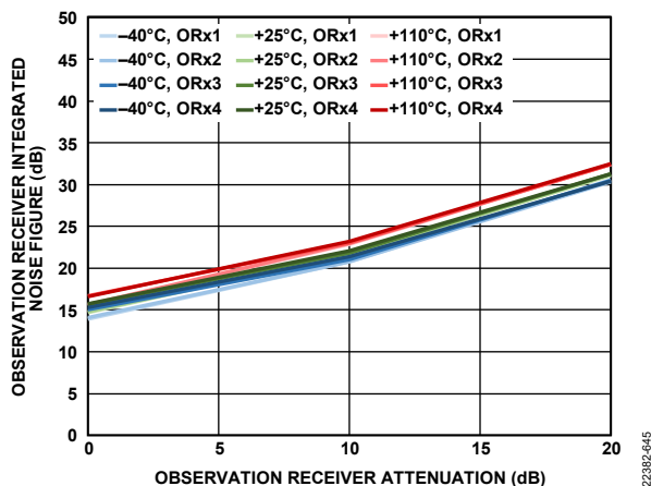
Figure 47. Observation Receiver (ORx) Integrated Noise Figure vs. Observation Receiver Attenuation, 141 MHz Bandwidth, Sample Rate = 153.6 MSPS, Integration Bandwidth = 500 kHz to 245.76 MHz
