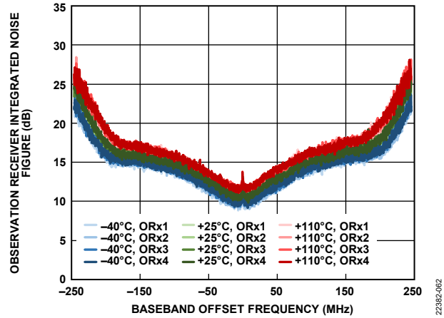
Figure 133. Observation Receiver Integrated Noise Figure vs. Baseband Offset Frequency, 450 MHz Bandwidth, Sample Rate = 491.52 MSPS, Integrated in 200 kHz Steps
