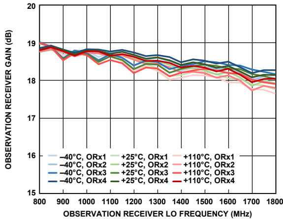
Figure 136. Observation Receiver Gain vs. Observation Receiver LO Frequency, 450 MHz Bandwidth, Sample Rate = 491.52 MSPS
