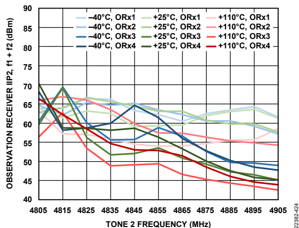
Figure 495. Observation Receiver IIP2, f_1 + f_2 vs. Tone 2 Frequency, Both Tones at -13 dBFS, f_1 = f_2 + 2 MHz
