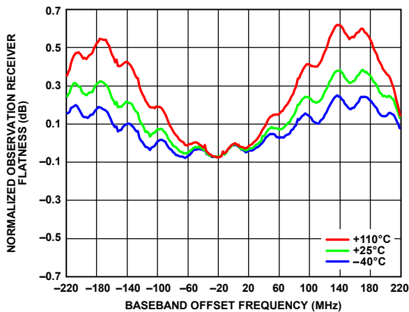
Figure 138. Normalized Observation Receiver Flatness vs. Baseband Offset Frequency, -10 dBFS Input Signal
