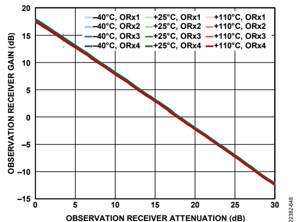
Figure 50. Observation Receiver Gain vs. Observation Receiver Attenuation, 45 MHz Offset, 141 MHz Bandwidth, Sample Rate = 153.6 MSPS
