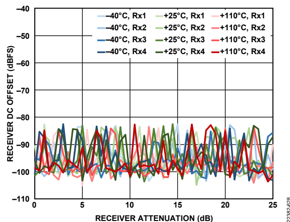
Figure 30. Receiver DC Offset vs. Receiver Attenuation, 10 MHz Offset, -5 dBFS Input Signal
