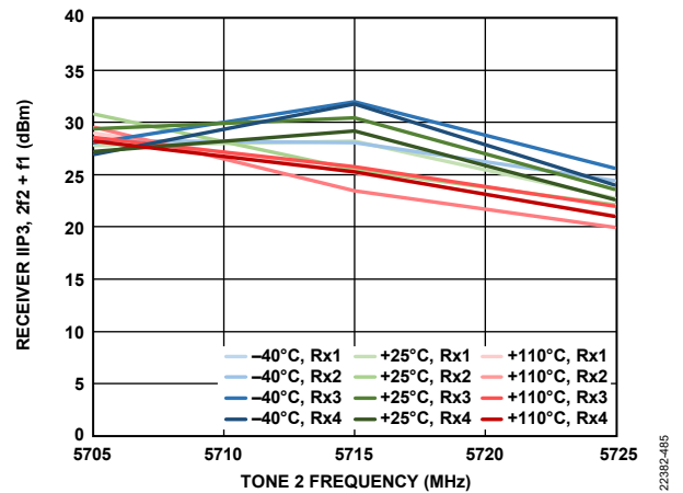
Figure 556. Receiver IIP3, 2f_2 + f_1 vs. Tone 2 Frequency, Both Tones at -11 dBFS, f_1 = f_2 + 2 MHz
