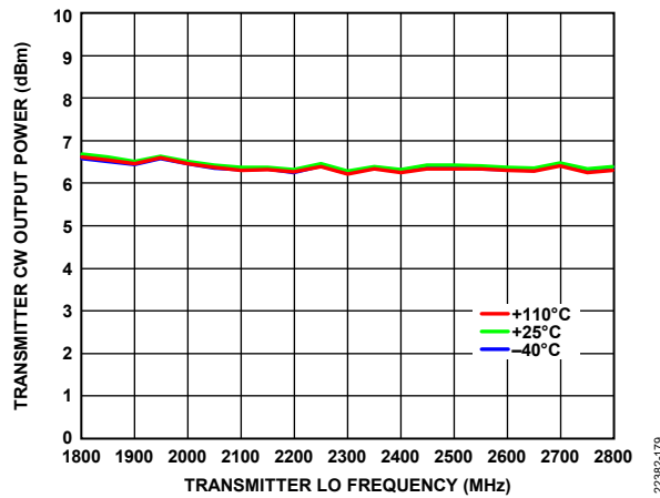
Figure 250. Transmitter Continuous Wave Output Power vs. Transmitter LO Frequency, 10 MHz Offset, 0 dB Attenuation
