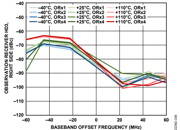
Figure 407. Observation Receiver HD3, Right Side vs. Baseband Offset Frequency, -10 dBFS Input Signal, Distortion Tone Measured Right of 0 Hz
