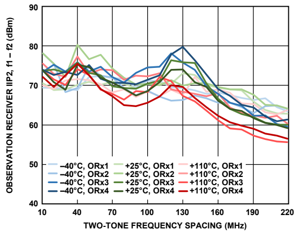
Figure 150. Observation Receiver IIP2, f_1 - f_2 vs. Two-Tone Frequency Spacing, Both Tones at -13 dBFS, f_2 = 2 MHz
