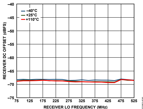
Figure 31. Receiver DC Offset vs. Receiver LO Frequency, 10 MHz Offset, -5 dBFS Input Signal
