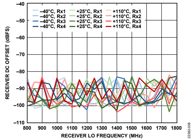
Figure 109. Receiver DC Offset vs. Receiver LO Frequency, 20 MHz Offset, -5 dBFS Input Signal
