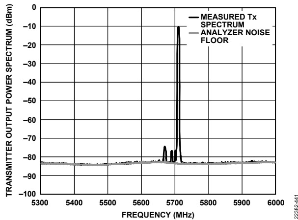
Figure 512. Transmitter Output Power Spectrum, Tx1, 5 MHz LTE, 10 MHz Offset, -10 dBFS RMS, 1 MHz Resolution Bandwidth, T j = 25°C
