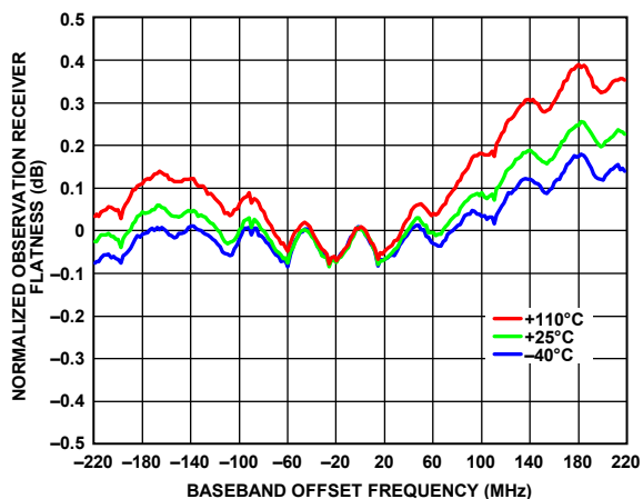
Figure 312. Normalized Observation Receiver Flatness vs. Baseband Offset Frequency, -10 dBFS Input Signal
