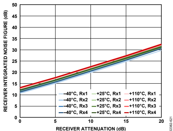
Figure 23. Receiver Integrated Noise Figure vs. Receiver Attenuation, 62.5 MHz Bandwidth, Sample Rate = 76.8 MSPS, Integration Bandwidth = 500 kHz to 100 MHz
