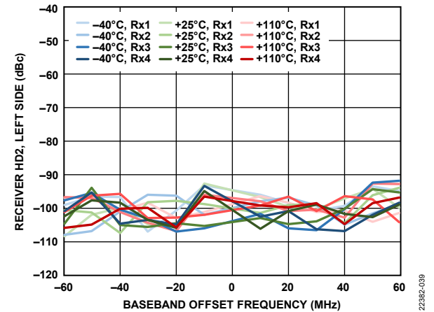
Figure 110. Receiver HD2, Left Side vs. Baseband Offset Frequency, -5 dBFS Input Signal, Distortion Tone Measured Left of 0 Hz (HD2 Canceller Enabled)
