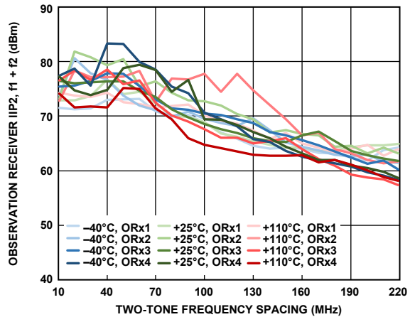
Figure 149. Observation Receiver IIP2, f_1 + f_2 vs. Two-Tone Frequency Spacing, Both Tones at -13 dBFS, f_2 = 2 MHz
