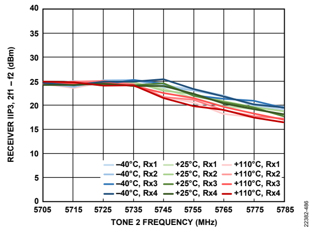
Figure 557. Receiver IIP3, 2f_1 - f_2 vs. Tone 2 Frequency, Both Tones at -11 dBFS, f_1 = f_2 + 2 MHz
