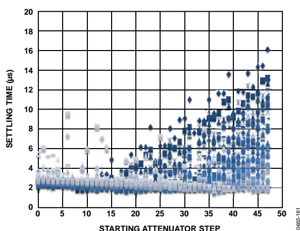
Figure 45. Attenuator Settling Time to 0.2 dB for Large Steps (7 dB to 47 dB) at Nominal Conditions
