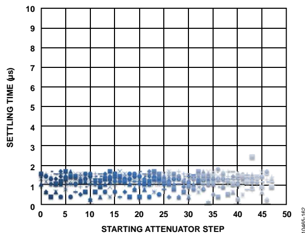
Figure 44. Attenuator Settling Time to 0.5 dB for Small Steps (1 dB to 6 dB) at Nominal Conditions
