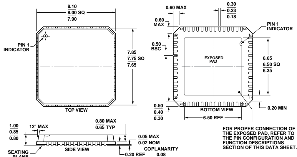
Figure 78. 56-Lead Lead Frame Chip Scale Package [LFCSP_VQ] 8 mm x 8 mm Body, Very Thin Quad (CP-56-4) Dimensions shown in millimeters
