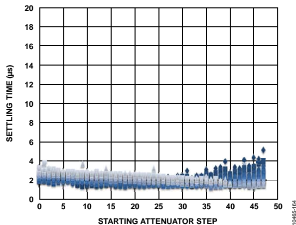
Figure 46. Attenuator Settling Time to 0.5 dB for Large Steps (7 dB to 47 dB) at Nominal Conditions
