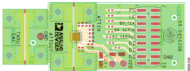
Figure 38. Evaluation Board, Top View
