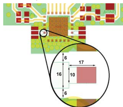
Figure 43. Without Impedance Match
