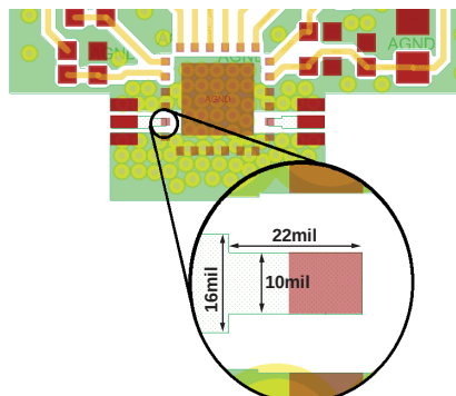
Figure 43. With Impedance Match
