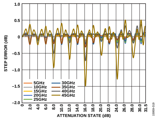
Figure 19. Step Error vs. Attenuation State over Frequency Without Impedance Match
