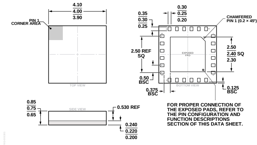
Figure 44. 24-Terminal Land Grid Array [LGA] 4 mm × 4 mm Body and 0.75 mm Package Height (CC-24-5) Dimensions shown in millimeters
