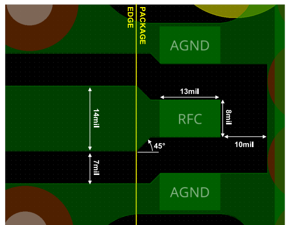
Figure 27. Recommended RF Pin Transitions
