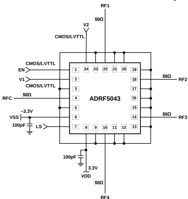
Figure 25. Application Circuit
