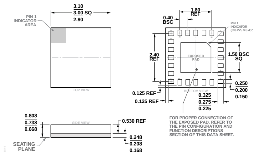
Figure 26. 24-Terminal Land Grid Array [LGA] 3 mm x 3 mm Body and 0.738 mm Package Height (CC-24-12) Dimensions shown in millimeters
