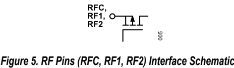
Figure 5. RF Pins (RFC, RF1, RF2) Interface Schematic
