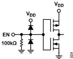
Figure 9. EN Pin Interface Schematic
