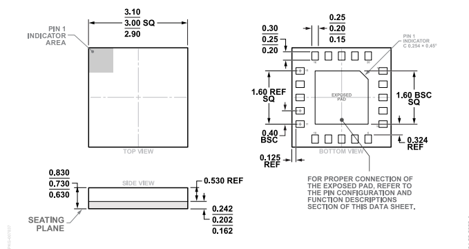
Figure 22. 20-Terminal Land Grid Array [LGA] 3.0 mm × 3.0 mm Body and 0.730 mm Package Height (CC-20-19) Dimensions shown in millimeters
