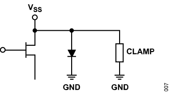
Figure 7. V SS Pin Interface Schematic
