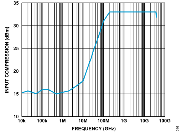
Figure 16. 0.1 dB Input Compression vs. Frequency, Low-Frequency Detail
