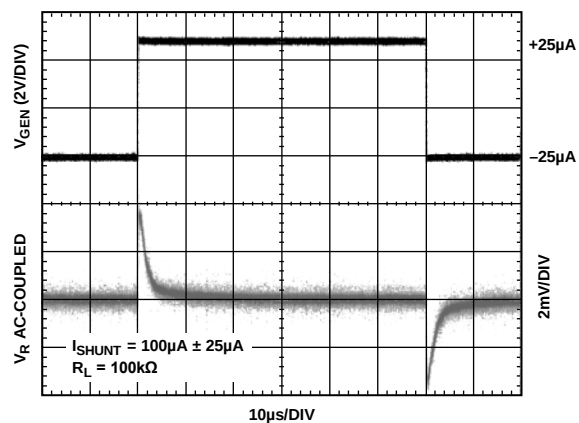
Figure 8. ADR5041 Load Transient Response
