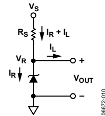
Figure 10. Typical Connection Diagram
