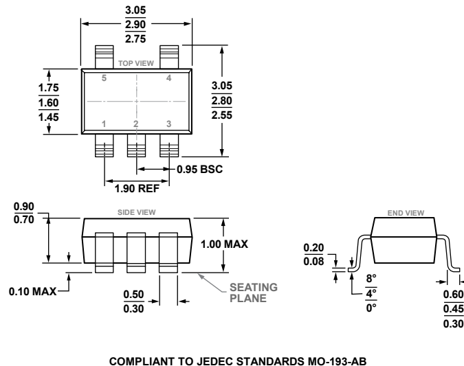
Figure 47. 5-Lead Thin Small Outline Transistor Package [TSOT] (UJ-5)
