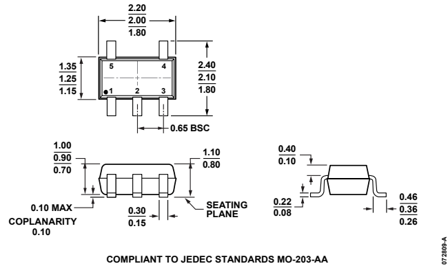
Figure 46. 5-Lead Thin Shrink Small Outline Transistor Package [SC70] (KS-5)
