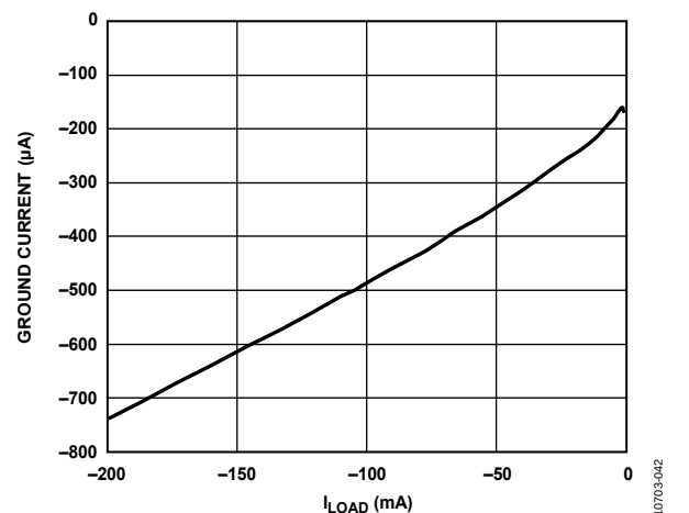
Figure 44. Ground Current vs. Load Current ( I_{LOAD} ), Adjustable Output Voltage, V_{OUT} = -15 V
