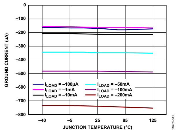
Figure 43. Ground Current vs. Junction Temperature ( T_J ), Adjustable Output Voltage, V_{OUT} = -15 V
