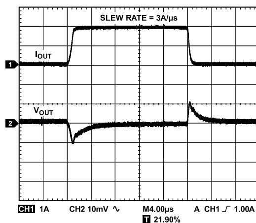
Figure 33. Load Transient Response, I_{LOAD} = 100\text{ mA} to 2\text{ A} , V_{OUT} = 3.3\text{ V} , V_{IN} = 4.0\text{ V} , Channel 1 = I_{OUT} , Channel 2 = V_{OUT}
