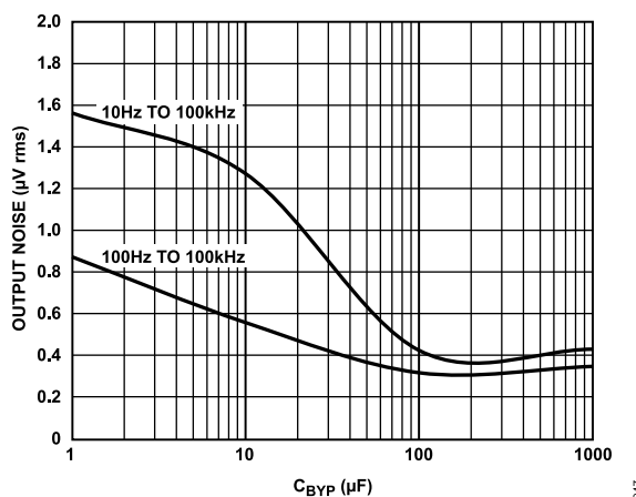
Figure 45. RMS Output Noise vs. Bypass Capacitance ( C_{\text{BYP}} )
