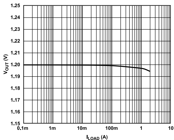
Figure 16. Output Voltage ( V_{OUT} ) vs. Load Current ( I_{LOAD} ), V_{OUT} = 1.2\text{ V}
