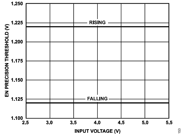
Figure 51. Typical EN Threshold vs. Input Voltage ( V_{IN} )
