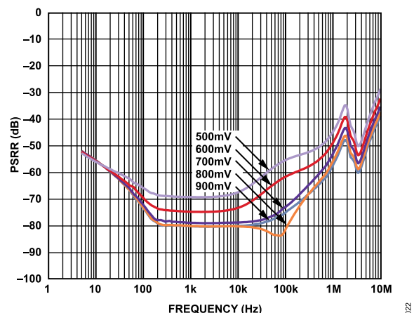
Figure 22. Power Supply Rejection Ratio (PSRR) vs. Frequency at Various Headroom Voltages, V_{OUT} = 3.3\text{ V} , 2 A Load
