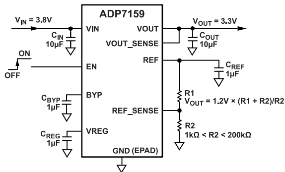
Figure 42. Typical Adjustable Output Voltage Application Schematic
