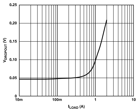
Figure 12. Dropout Voltage ( V_{DROPOUT} ) vs. Load Current ( I_{LOAD} ), V_{OUT} = 3.3\text{ V}
