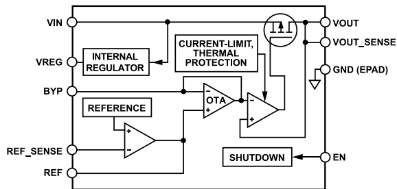
Figure 41. Simplified Internal Block Diagram
