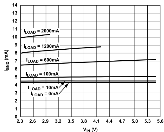
Figure 20. Ground Current ( I_{GND} ) vs. Input Voltage ( V_{IN} ) at Various Loads, V_{OUT} = 1.2\text{ V}
