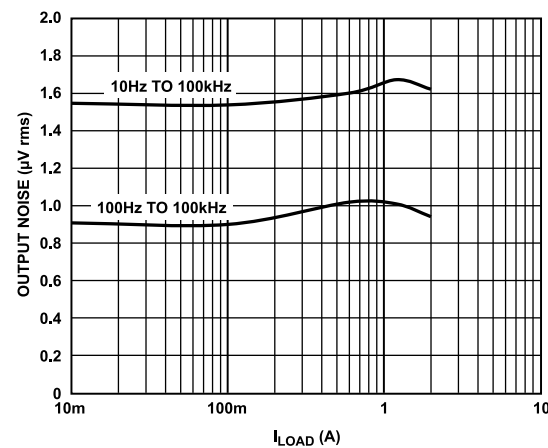
Figure 28. RMS Output Noise vs. Load Current ( I_{LOAD} )
