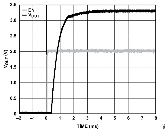
Figure 50. Typical VOUT Response to EN Pin Operation ( V_{EN} ), V_{OUT} = 3.3 V, V_{IN} = 5 V, C_{BYP} = 1 \mu F
