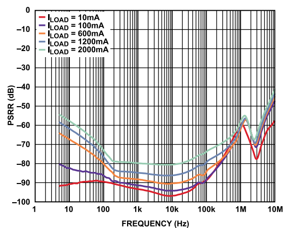
Figure 24. Power Supply Rejection Ratio (PSRR) vs. Frequency at Various Loads, V_{OUT} = 1.2\text{ V} , V_{IN} = 2.4\text{ V}
