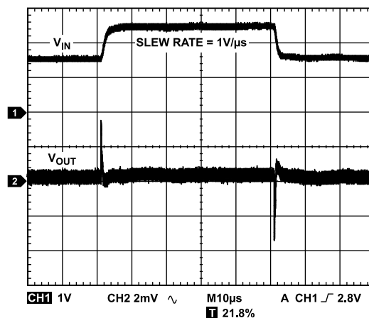
Figure 38. Line Transient Response, 1\text{ V} Input Step, I_{LOAD} = 2\text{ A} , V_{OUT} = 1.8\text{ V} , V_{IN} = 2.5\text{ V} , Channel 1 = V_{IN} , Channel 2 = V_{OUT}
