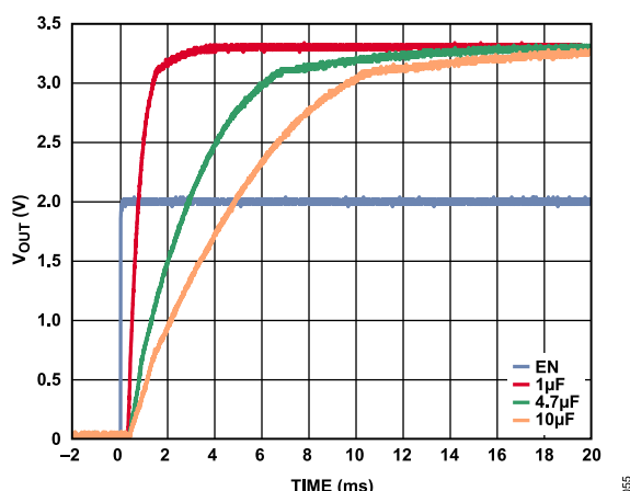
Figure 53. Typical Start-Up Behavior with C_{BYP} = 1 \mu F to 10 \mu F
