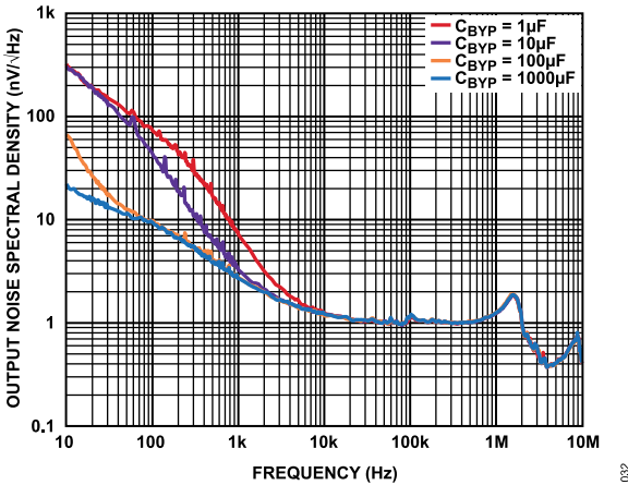
Figure 2. Noise Spectral Density at Different Values of C_{BYP} , V_{OUT} = 3.3 V
