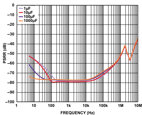
Figure 27. Power Supply Rejection Ratio (PSRR) vs. Frequency at Various C_{BYF} Values, V_{OUT} = 3.3\text{ V} , V_{IN} = 4.0\text{ V} , 2 A Load
