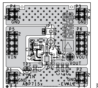
Figure 64. Sample 8-Lead SOIC PCB Layout
