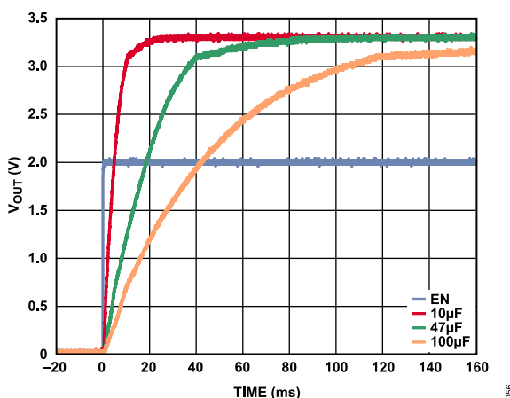
Figure 54. Typical Start-Up Behavior with C_{BYP} = 10 \mu F to 100 \mu F
