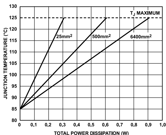
Figure 57. Junction Temperature vs. Total Power Dissipation for the 10-Lead LFCSP, T_A = 85^\circ\text{C}
