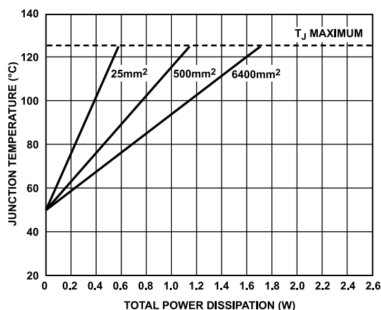
Figure 56. Junction Temperature vs. Total Power Dissipation for the 10-Lead LFCSP, T_A = 50^\circ\text{C}
