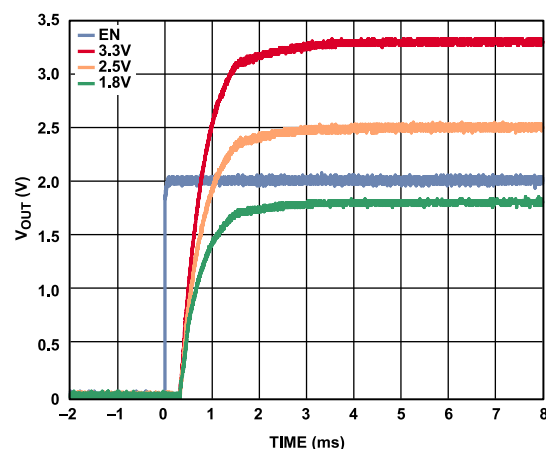
Figure 39. V_{OUT} Start-Up Time After V_{EN} Rising at Various Output Voltages, V_{IN} = 5.0\text{ V} , C_{BYP} = 1\text{ μF}
