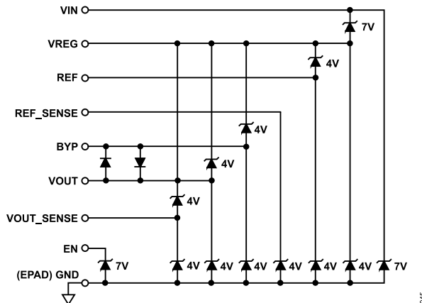
Figure 43. Simplified ESD Protection Block Diagram
