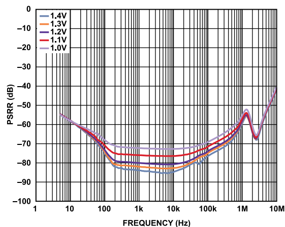
Figure 25. Power Supply Rejection Ratio (PSRR) vs. Frequency at Various Headroom Voltages, V_{OUT} = 1.2\text{ V} , 2 A Load
