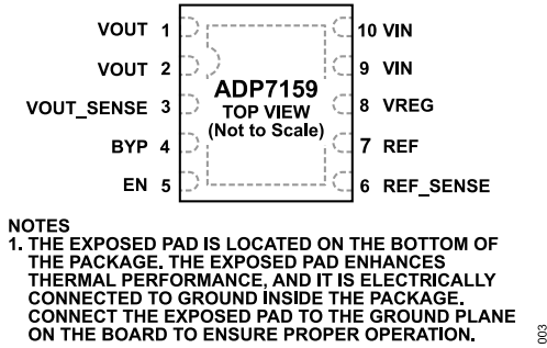
Figure 3. 10-Lead LFCSP Pin Configuration
