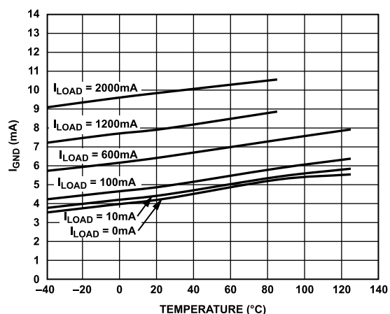
Figure 18. Ground Current ( I_{GND} ) vs. Temperature at Various Loads, V_{OUT} = 1.2\text{ V}
