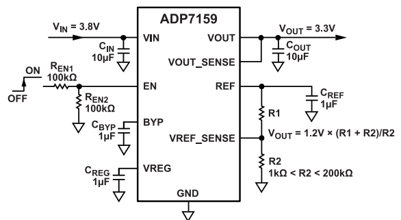
Figure 52. Typical EN Pin Voltage Divider
