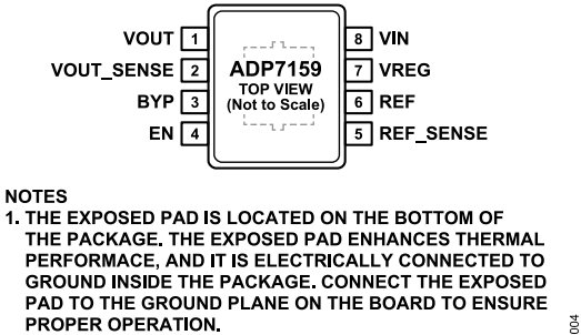
Figure 4. 8-Lead SOIC Pin Configuration
