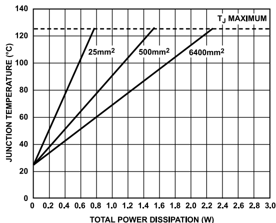
Figure 55. Junction Temperature vs. Total Power Dissipation for the 10-Lead LFCSP, T_A = 25^\circ\text{C}
