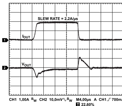
Figure 34. Load Transient Response, I_{LOAD} = 100\text{ mA} to 2\text{ A} , V_{OUT} = 3.3\text{ V} , V_{IN} = 4.0\text{ V} , C_{OUT} = 22\mu\text{F} , Channel 1 = I_{OUT} , Channel 2 = V_{OUT}
