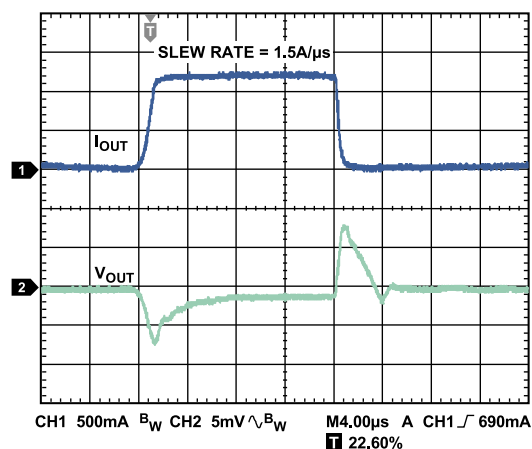
Figure 33. Load Transient Response, I_{\text{LOAD}} = 100\text{mA} to 1.2\text{A} , V_{\text{OUT}} = 3.3\text{V} , V_{\text{IN}} = 4.0\text{V} , C_{\text{OUT}} = 22\mu\text{F} , Channel 1 = I_{\text{OUT}} , Channel 2 = V_{\text{OUT}}
