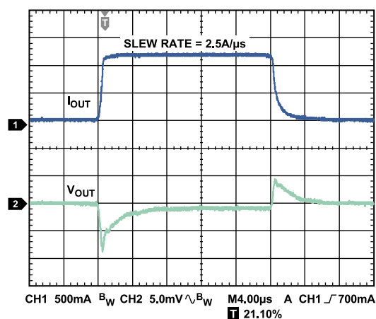
Figure 32. Load Transient Response, I_{\text{LOAD}} = 100\text{mA} to 1.2\text{A} , V_{\text{OUT}} = 3.3\text{V} , V_{\text{IN}} = 4.0\text{V} , Channel 1 = I_{\text{OUT}} , Channel 2 = V_{\text{OUT}}
