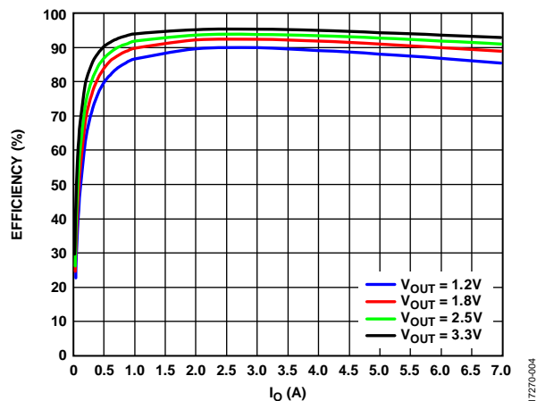
Figure 4. Channel 1/Channel 2 Efficiency Curve, V_{IN} = 5\text{ V} , f_{SW} = 600\text{ kHz} , FPWM Mode
