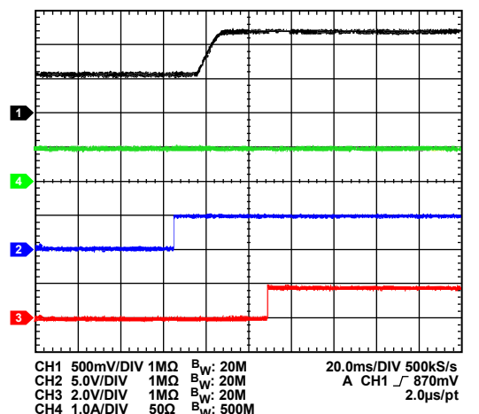
Figure 42. Channel 1 Startup with Precharged Output, V_{IN} = 12\text{ V} , V_{OUT} = 1.2\text{ V} , f_{SW} = 600\text{ kHz} , FPWM Mode, Channel 1 = V_{OUT} , Channel 2 = EN, Channel 3 = PWRGD, Channel 4 = I_{OUT}
