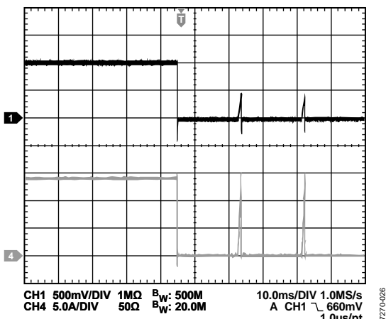
Figure 26. Channel 1/Channel 2 Short-Circuit Protection Entry, V_{IN} = 12\text{ V} , V_{OUT} = 1.0\text{ V} , f_{SW} = 600\text{ kHz} , L = 1\text{ µH} , C_{OUT} = 47\text{ µF} \times 6 , Channel 1 = V_{OUT} , Channel 4 = I_{OUT}
