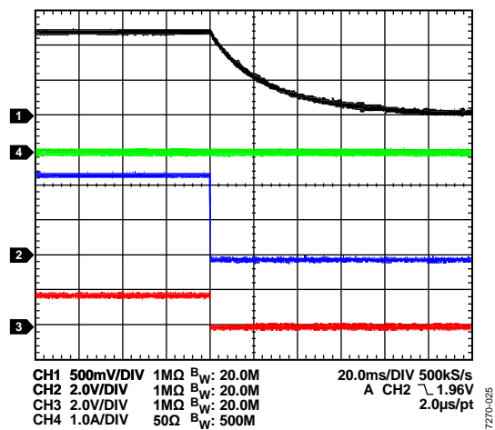
Figure 25. Channel 1/Channel 2 Shutdown with Active Output Discharge, V_{IN} = 12\text{ V} , V_{OUT} = 1.2\text{ V} , f_{SW} = 600\text{ kHz} , L = 1\text{ µH} , C_{OUT} = 47\text{ µF} \times 6 , Channel 1 = V_{OUT} , Channel 2 = EN , Channel 3 = PWRGD , Channel 4 = I_{OUT}
