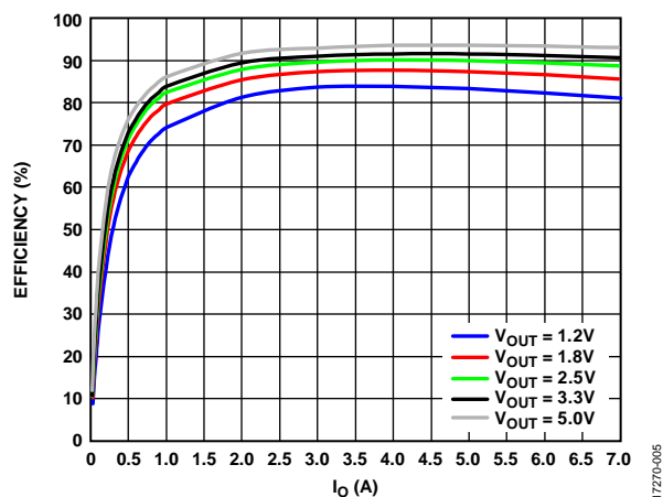
Figure 5. Channel 1/Channel 2 Efficiency Curve, V_{IN} = 12\text{ V} , f_{SW} = 600\text{ kHz} , FPWM Mode
