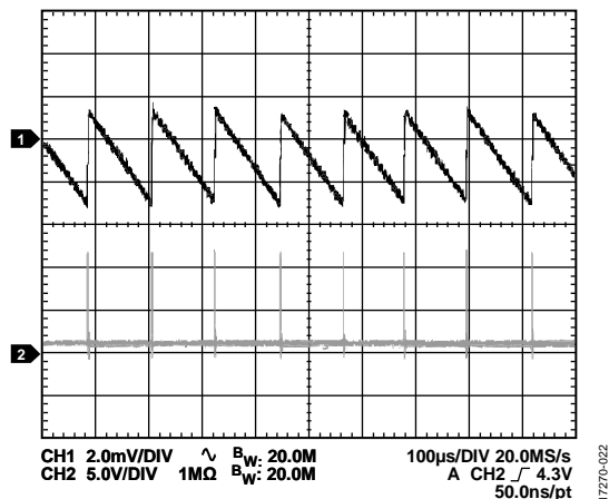
Figure 22. Channel 1/Channel 2 Steady State Waveform, V_{IN} = 12\text{ V} , V_{OUT} = 1.2\text{ V} , I_{OUT} = 10\text{ mA} , f_{SW} = 600\text{ kHz} , L = 1\text{ µH} , C_{OUT} = 47\text{ µF} \times 6 , Automatic PWM/PSM, Channel 1 = V_{OUT} , Channel 2 = SW
