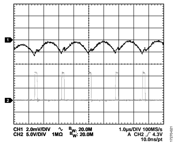
Figure 21. Channel 1/Channel 2 Steady State Waveform, V_{IN} = 12 V , V_{OUT} = 1.2 V , I_{OUT} = 7 A , f_{SW} = 600 kHz , L = 1 \mu H , C_{OUT} = 47 \mu F \times 6 , FPWM Mode, Channel 1 = V_{OUT} , Channel 2 = Switching Point (SW)
