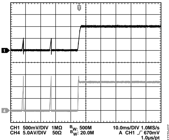
Figure 27. Channel 1/Channel 2 Short-Circuit Protection Recovery, V_{IN} = 12\text{ V} , V_{OUT} = 1.0\text{ V} , f_{SW} = 600\text{ kHz} , L = 1\text{ µH} , C_{OUT} = 47\text{ µF} \times 6 , Channel 1 = V_{OUT} , Channel 4 = I_{OUT}
