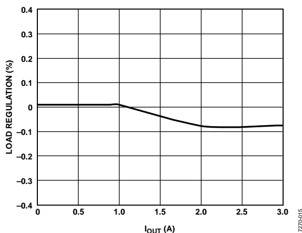
Figure 15. Channel 3 Load Regulation, V_{IN} = 12\text{ V} , V_{OUT} = 1.2\text{ V} , f_{SW} = 600\text{ kHz} , FPWM Mode
