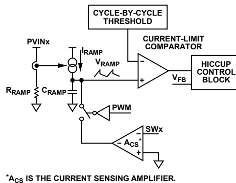
Figure 43. Current-Limit Circuitry
