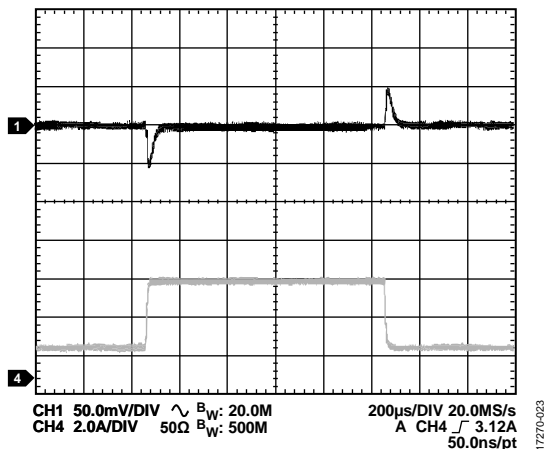
Figure 23. Load Transient, Channel 1/Channel 2 from 1.5 A to 5 A, V_{IN} = 12\text{ V} , V_{OUT} = 3.3\text{ V} , f_{SW} = 600\text{ kHz} , L = 1\text{ µH} , C_{OUT} = 47\text{ µF} \times 6 , 1 A/µs, Channel 1 = V_{OUT} , Channel 4 = I_{OUT}
