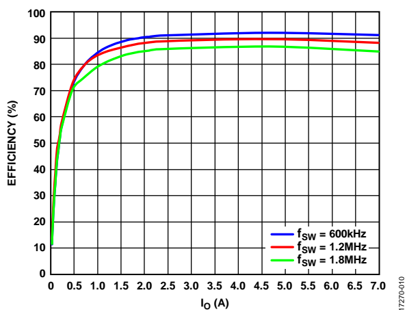
Figure 10. Channel 1/Channel 2 Efficiency Curve, V_{IN} = 12\text{ V} , Output Voltage ( V_{OUT} ) = 3.3 V, FPWM Mode (600 kHz, 1.2 MHz, 1.8 MHz)
