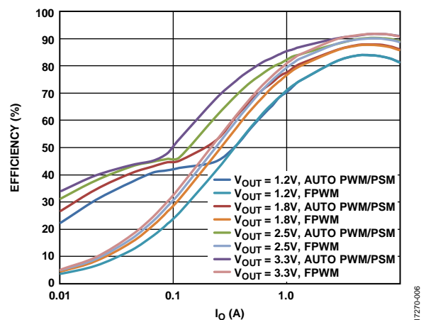
Figure 6. Channel 1/Channel 2 Efficiency Curve, V_{IN} = 12\text{ V} , f_{SW} = 600\text{ kHz} , FPWM and Automatic PWM/PSM Modes
