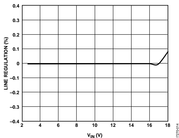
Figure 14. Channel 3 Line Regulation, V_{OUT} = 1.2\text{ V} , I_{OUT} = 3\text{ A} , f_{SW} = 600\text{ kHz} , FPWM Mode
