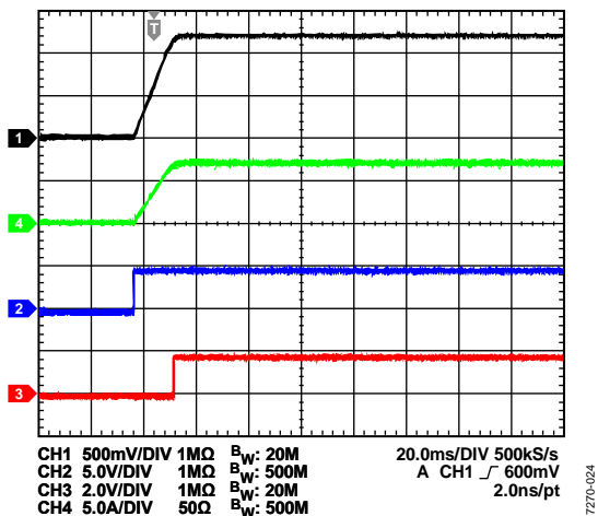
Figure 24. Channel 1/Channel 2 Soft Start with 7 A Resistance Load, V_{IN} = 12\text{ V} , V_{OUT} = 1.2\text{ V} , f_{SW} = 600\text{ kHz} , L = 1\text{ µH} , C_{OUT} = 47\text{ µF} \times 6 , Channel 1 = V_{OUT} , Channel 2 = EN , Channel 3 = PWRGD , Channel 4 = I_{OUT}
