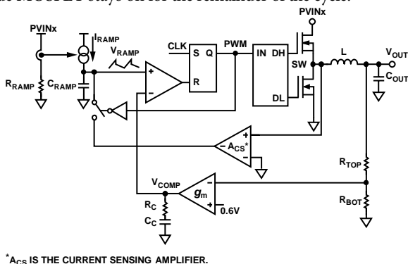
Figure 28. FlexMode™ PWM Control Architecture
