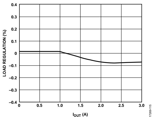
Figure 16. Channel 3 Load Regulation, V_{IN} = 12\text{ V} , V_{OUT} = 1.2\text{ V} , f_{SW} = 600\text{ kHz} , FPWM Mode
