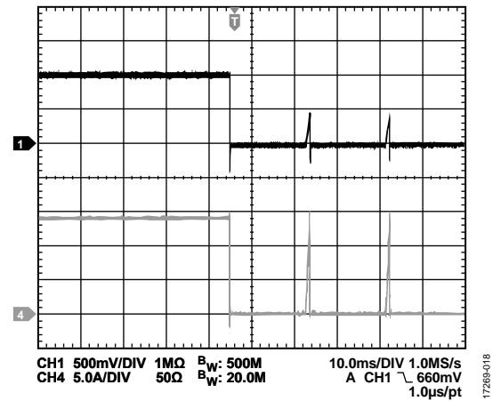
Figure 27. Channel 1/Channel 2 Short-Circuit Protection Entry, V_{IN} = 12\text{ V} , V_{OUT} = 1.0\text{ V} , f_{SW} = 600\text{ kHz} , L = 1\text{ µH} , C_{OUT} = 47\text{ µF} \times 6 , Channel 1 = V_{OUT} , Channel 4 = I_{OUT}
