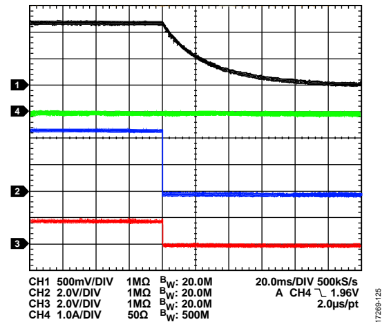
Figure 26. Channel 1/Channel 2 Shutdown with Active Output Discharge, V_{IN} = 12\text{ V} , V_{OUT} = 1.2\text{ V} , f_{SW} = 600\text{ kHz} , L = 1\text{ µH} , C_{OUT} = 47\text{ µF} \times 6 , Channel 1 = V_{OUT} , Channel 2 = EN , Channel 3 = PWRGD , Channel 4 = I_{OUT}
