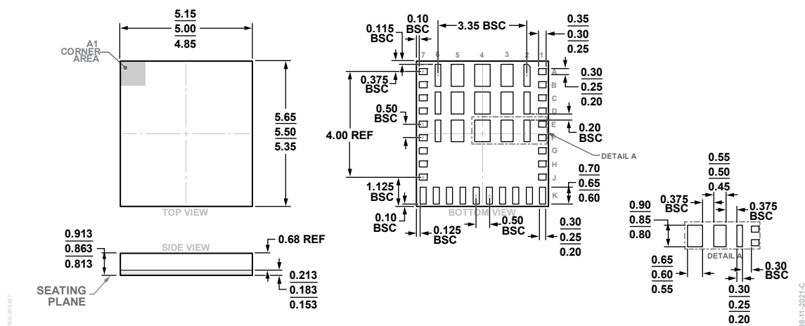
Figure 58. 43-Terminal Land Grid Array [LGA] (CC-43-1)
