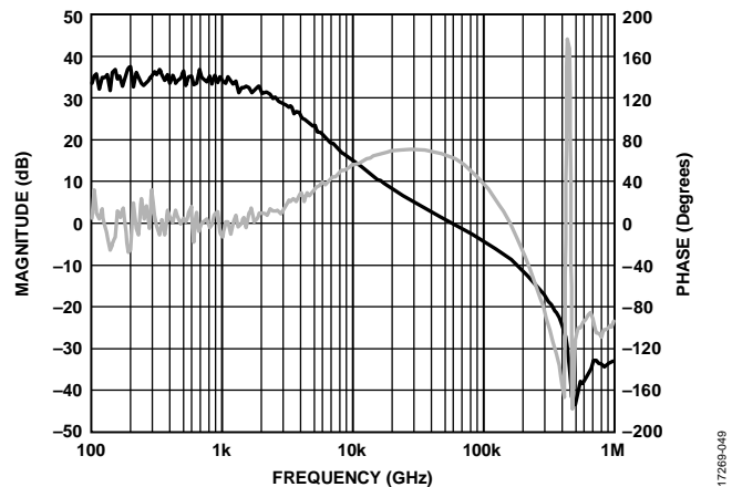
Figure 56. Bode Plot for 1.2 V Output
