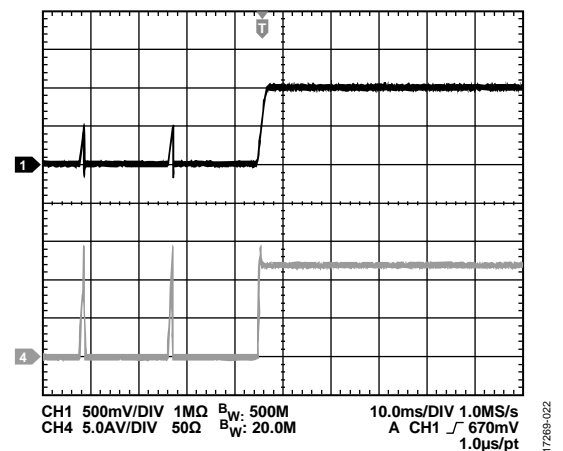
Figure 28. Channel 1/Channel 2 Short-Circuit Protection Recovery, V_{IN} = 12\text{ V} , V_{OUT} = 1.0\text{ V} , f_{SW} = 600\text{ kHz} , L = 1\text{ µH} , C_{OUT} = 47\text{ µF} \times 6 , Channel 1 = V_{OUT} , Channel 4 = I_{OUT}
