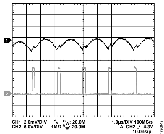
Figure 22. Channel 1/Channel 2 Steady State Waveform, V_{IN} = 12V , V_{OUT} = 1.2V , I_{OUT} = 7A , f_{SW} = 600kHz , L = 1\mu H , C_{OUT} = 47\mu F \times 6 , FPWM Mode, Channel 1 = V_{OUT} , Channel 2 = Switching Point (SW)
