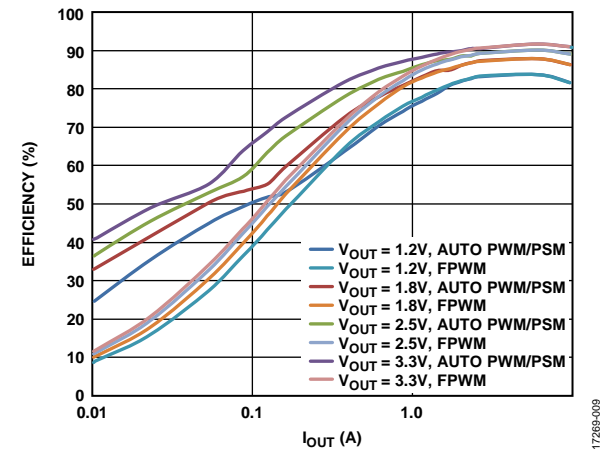
Figure 10. Channel 3 Efficiency Curve, V_{IN} = 12\text{ V} , f_{SW} = 600\text{ kHz} , FPWM Mode and Automatic PWM/PSM Modes
