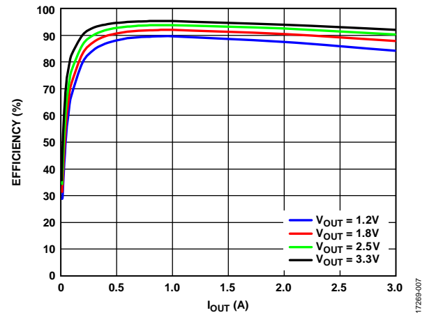
Figure 8. Channel 3 Efficiency Curve, V_{IN} = 5\text{ V} , f_{SW} = 600\text{ kHz} , FPWM Mode
