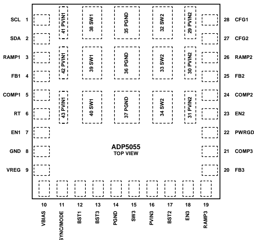
Figure 4. Pin Configuration
