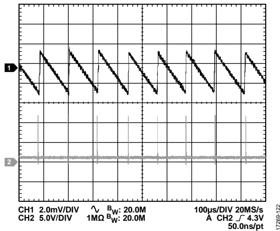
Figure 23. Channel 1/Channel 2 Steady State Waveform, V_{IN} = 12\text{ V} , V_{OUT} = 1.2\text{ V} , I_{OUT} = 10\text{ mA} , f_{SW} = 600\text{ kHz} , L = 1\text{ µH} , C_{OUT} = 47\text{ µF} \times 6 , Automatic PWM/PSM, Channel 1 = V_{OUT} , Channel 2 = SW
