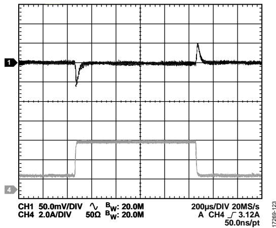
Figure 24. Load Transient, Channel 1/Channel 2 From 1.5 A to 5 A, V_{IN} = 12\text{ V} , V_{OUT} = 3.3\text{ V} , f_{SW} = 600\text{ kHz} , L = 1\text{ µH} , C_{OUT} = 47\text{ µF} \times 6 , 1 A/µs, Channel 1 = V_{OUT} , Channel 4 = I_{OUT}
