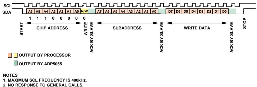
Figure 50. PMBus Write to Register
