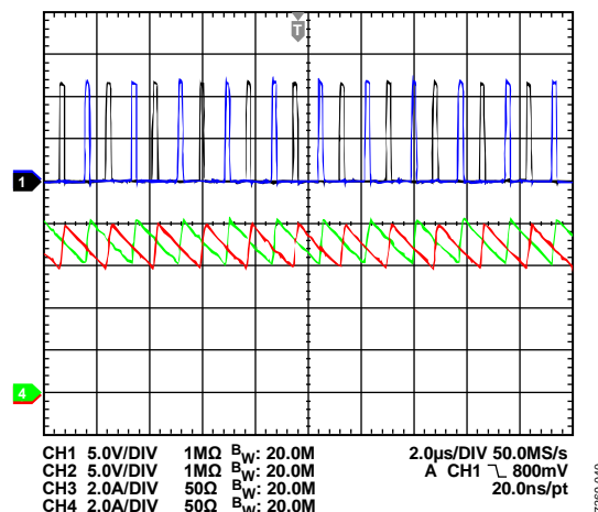
Figure 43. Steady State Waveform in Interleaved Parallel Output Configuration, V_{IN} = 12\text{ V} , V_{OUT} = 1.2\text{ V} , f_{SW} = 600\text{ kHz} , FPWM Mode, Channel 1 = SW1, Channel 2 = SW2, Channel 3 = Inductor Current of L1 ( I_{L1} ), Channel 4 = Inductor Current of L2 ( I_{L2} )
