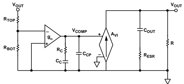
Figure 52. Simplified Peak Current Mode Control Small Signal Circuit
