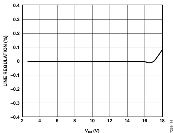
Figure 15. Channel 3 Line Regulation, V_{OUT} = 1.2\text{ V} , I_{OUT} = 3\text{ A} , f_{SW} = 600\text{ kHz} , FPWM Mode
