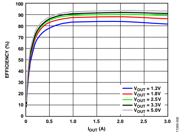
Figure 9. Channel 3 Efficiency Curve, V_{IN} = 12\text{ V} , f_{SW} = 600\text{ kHz} , FPWM Mode
