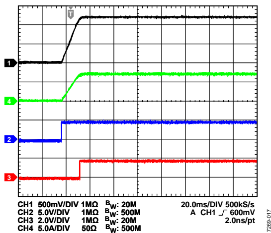
Figure 25. Channel 1/Channel 2 Soft Start with 7 A Resistance Load, V_{IN} = 12\text{ V} , V_{OUT} = 1.2\text{ V} , f_{SW} = 600\text{ kHz} , L = 1\text{ µH} , C_{OUT} = 47\text{ µF} \times 6 , Channel 1 = V_{OUT} , Channel 2 = EN , Channel 3 = PWRGD , Channel 4 = I_{OUT}
