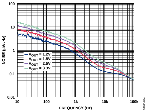
Figure 24. Channel 5 (LDO Regulator) Output Noise Spectrum, V_{IN} = 5\text{ V} , C_{OUT} = 1\text{ }\mu\text{F} , I_{OUT} = 10\text{ mA}
