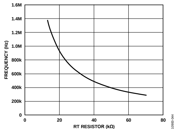
Figure 39. Switching Frequency vs. RT Resistor
