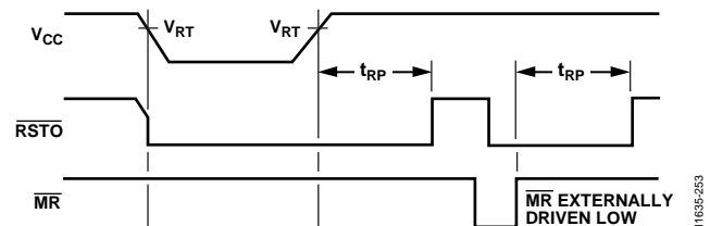
Figure 53. \overline{MR} Timing Diagram in Processor Reset Mode
