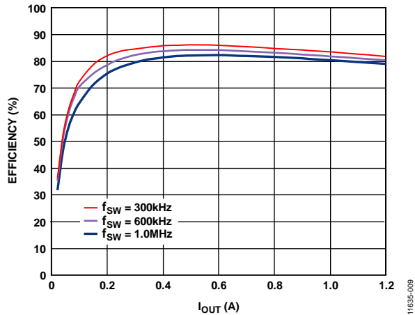
Figure 11. Channel 3/Channel 4 Efficiency Curve, V_{IN} = 12\text{ V} , V_{OUT} = 1.8\text{ V} , FPWM Mode
