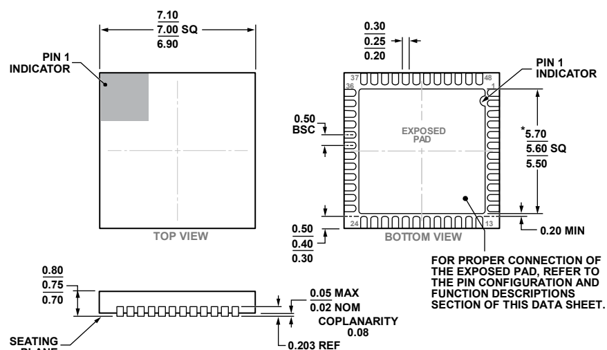
Figure 67. 48-Lead Lead Frame Chip Scale Package [LFCSP_WQ] 7 mm × 7 mm Body, Very Very Thin Quad (CP-48-13)
