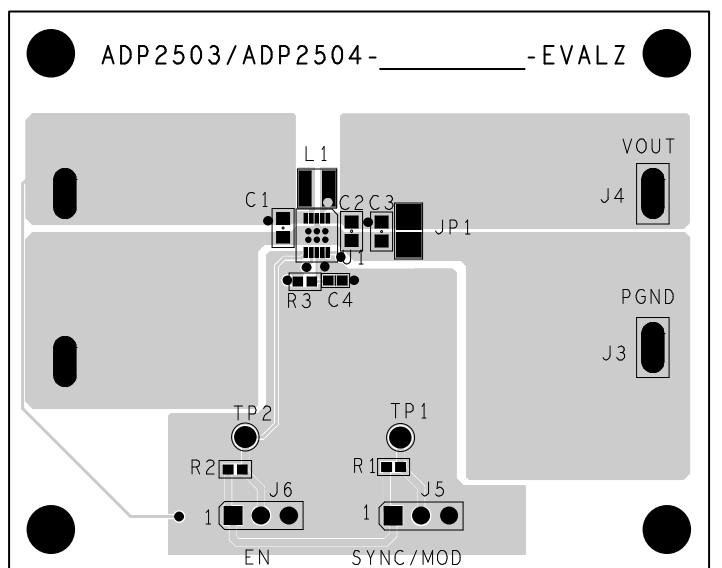
Figure 31. ADP2503/ADP2504 Evaluation Board for Fixed Output Voltages
