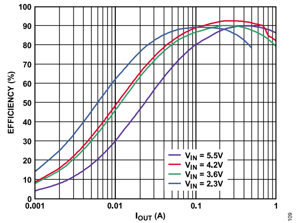
Figure 7. Efficiency vs. Output Current, PWM Mode ( V_{OUT} = 3.3 V)
