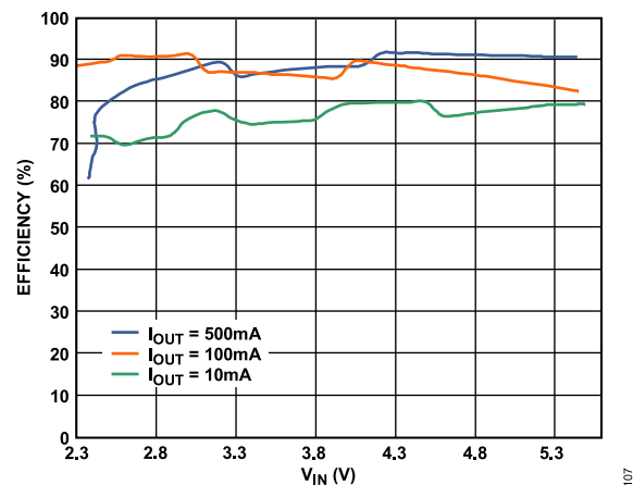
Figure 11. Efficiency vs. Input Voltage ( V_{OUT} = 3.3 V)
