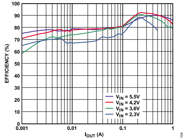
Figure 6. Efficiency vs. Output Current, PSM and PWM Mode ( V_{OUT} = 5.0 V)
