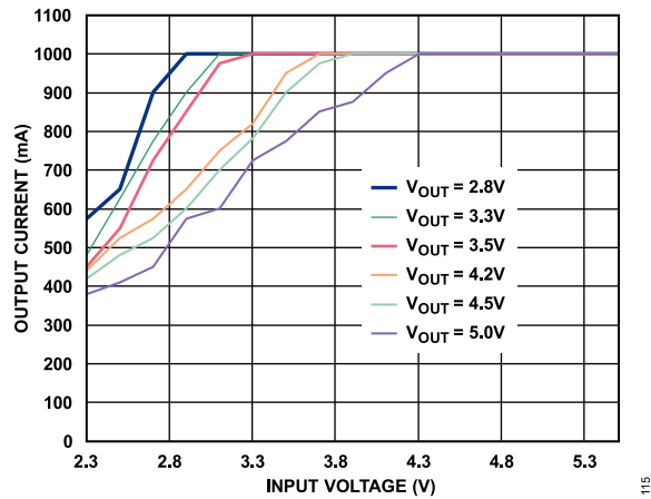
Figure 4. ADP2504 Output Current vs. Input Voltage
