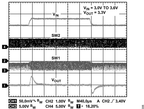
Figure 16. Line Transient, PWM Mode ( V_{IN} = 3.0 V to 3.6 V, V_{OUT} = 3.3 V)
