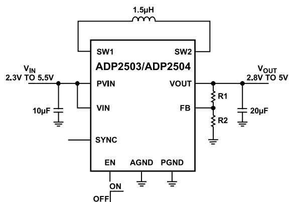
Figure 30. Typical Application Circuit for the Adjustable ADP2503/ADP2504
