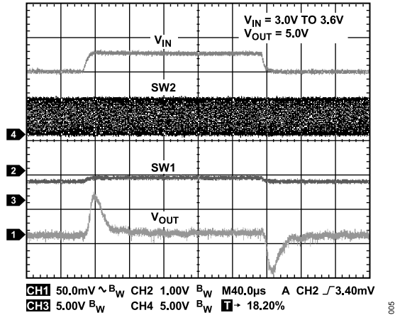
Figure 15. Line Transient, PWM Mode ( V_{IN} = 3.0 V to 3.6 V, V_{OUT} = 5.0 V)
