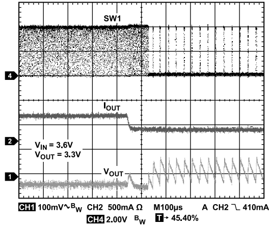
Figure 21. Mode Change by Load Transients, Load Fall ( V_{OUT} = 3.3\text{ V} )
