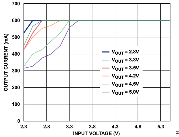
Figure 3. ADP2503 Output Current vs. Input Voltage
