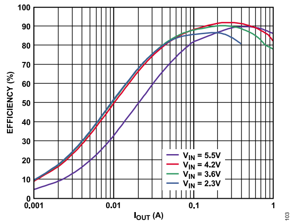
Figure 5. Efficiency vs. Output Current, PWM Mode ( V_{OUT} = 5.0 V)
