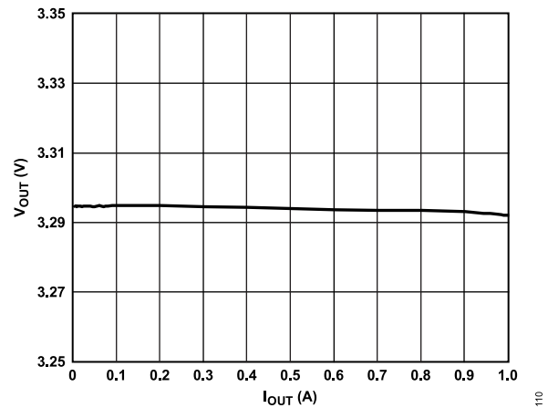
Figure 12. Load Regulation ( V_{IN} = 3.6 V, V_{OUT} = 3.3 V)
