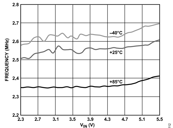
Figure 13. Frequency vs. Input Voltage Over Temperature ( V_{OUT} = 3.3 V)
