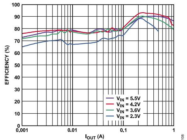
Figure 8. Efficiency vs. Output Current, PSM and PWM Mode ( V_{OUT} = 3.3 V)
