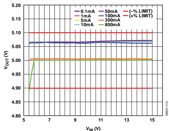
Figure 13. Line Regulation, V_{OUT} = 5.0\text{ V} , Different Loads
