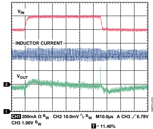
Figure 33. Line Transient, V_{OUT} = 3.3 V, PWM Mode, 800 mA, V_{IN1} = 6 V to 7 V, 2 µs Rise Time, C_{IN} = 3.3 µF
