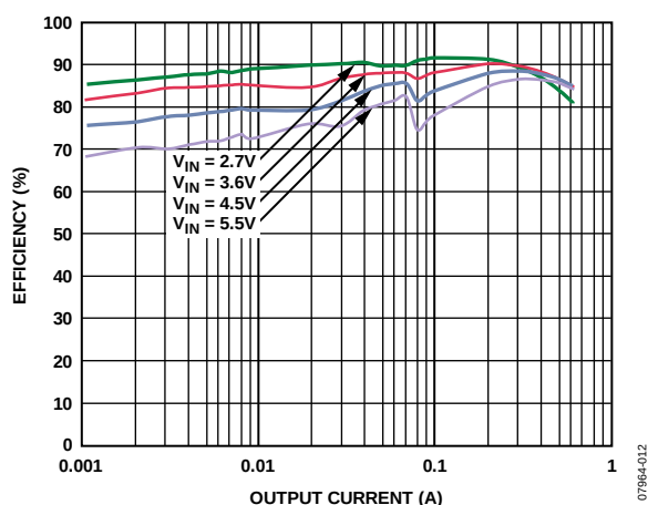
Figure 11. Efficiency, V_{OUT} = 1.8\text{ V}
