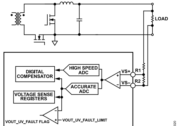
Figure 18. Voltage Sense Configuration
