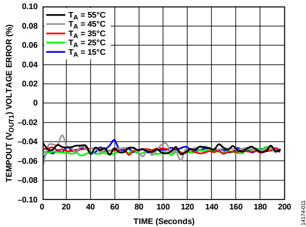
Figure 11. Thermal Stability (TEMPOUT) Voltage Error at Various Ambient Temperatures, V_{IN} = 3.3\text{ V} , V_{TEMPSET} = 1\text{ V}
