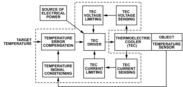
Figure 40. System Block Diagram
