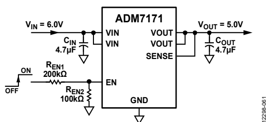
Figure 59. Typical EN Pin Voltage Divider
