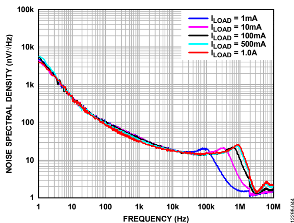
Figure 44. Output Noise Spectral Density, Adjustable Version, V_{OUT} = 1.2\text{ V}
