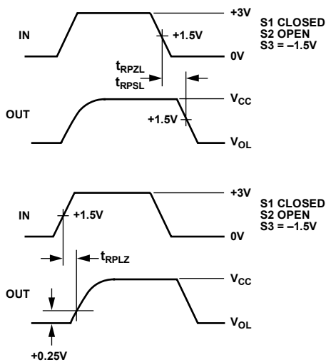
Figure 15. Receiver Enable and Disable Times
