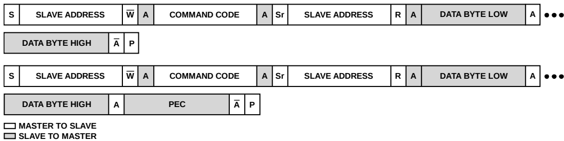
Figure 35. Read Word and Read Word with PEC
