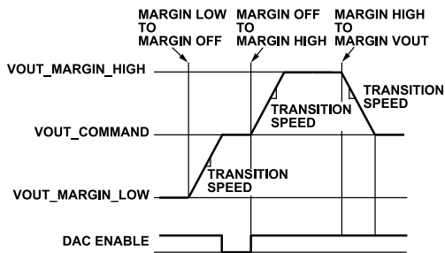
Figure 14. Margining Example 2
