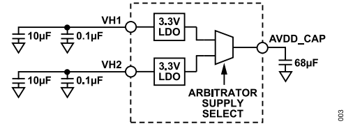
Figure 7. AVDD_CAP Arbitrator Operation
