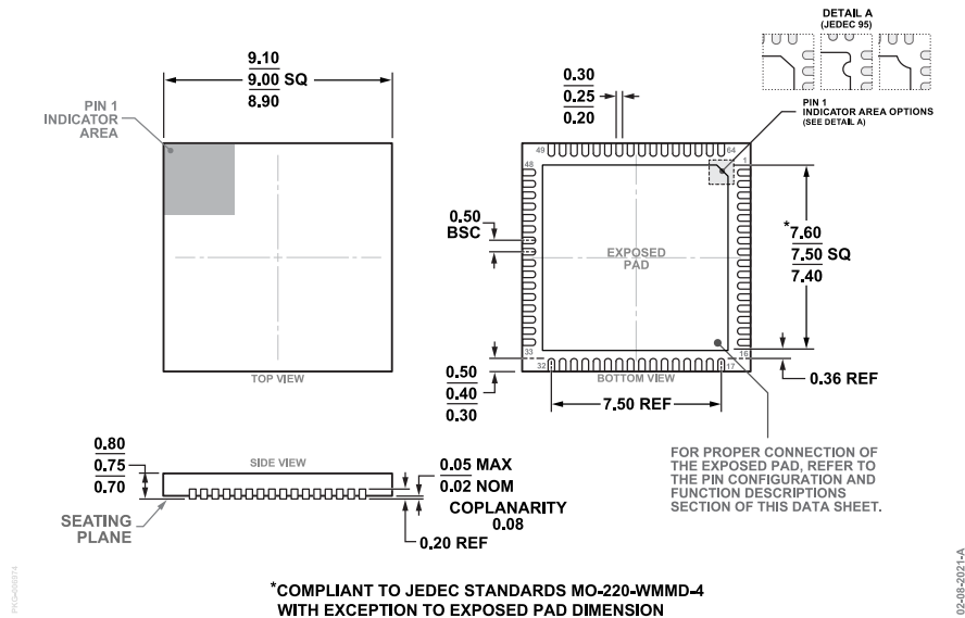
Figure 30. 64-Lead Lead Frame Chip Scale Package [LFCS] 9 mm x 9 mm Body and 0.75 mm Package Height (CP-64-23) Dimensions shown in millimeters
