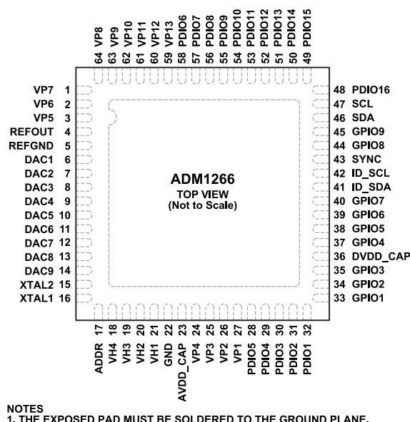
Figure 3. Pin Configuration
