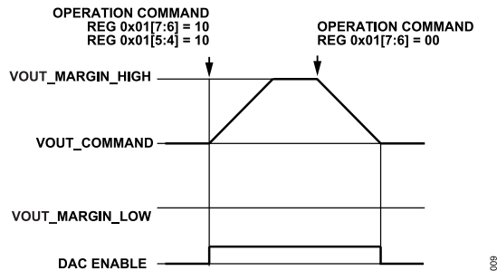
Figure 13. Margining Example 1
