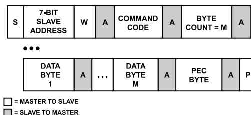
Figure 25. Block Write Protocol with PEC
