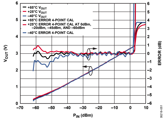
Figure 51. 2.14 GHz Transfer Function and Error at +25^{\circ}\text{C} , -40^{\circ}\text{C} , and +85^{\circ}\text{C} Using a Four-Point Calibration (0 dBm, -20 dBm, -45 dBm, -60 dBm)
