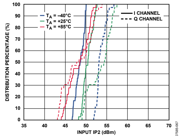
Figure 67. IIP2 Distributions for I Channel and Q Channel
