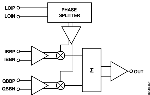
Figure 22. Block Diagram
