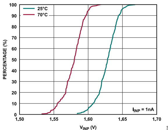
Figure 33. Input Voltage Distribution at I_{INP} = 1 \text{ nA}
