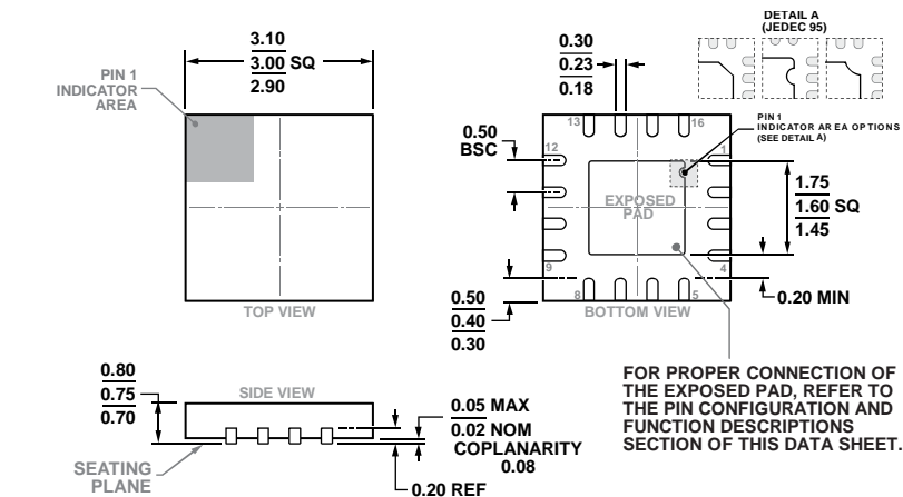
Figure 34. 16-Lead Lead Frame Chip Scale Package [LFCSP] 3 mm × 3 mm Body and 0.75 mm Package Height (CP-16-22)
