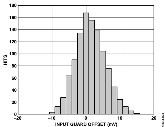
Figure 24. Distribution of Input Guard Offset Voltage V_{OLFS} ( V_{INPT} - V_{SUM} )
