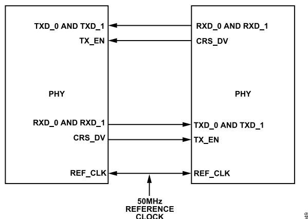
Figure 34. Back to Back with RMII Interface
