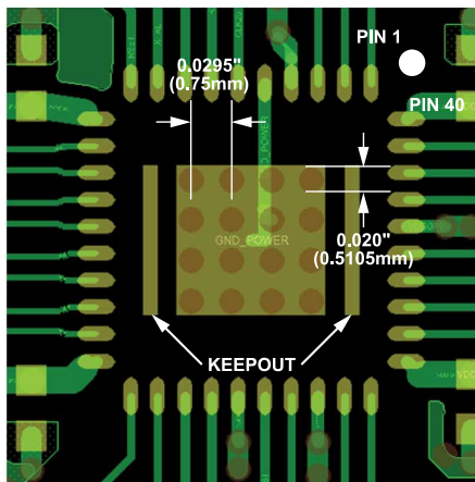
Figure 45. Exposed Paddle Via Array on EVAL-ADIN1300FMCZ
