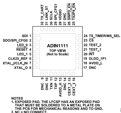
Figure 4. Pin Configuration
