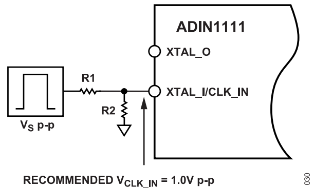
Figure 25. External 25 MHz Clock Input Circuit
