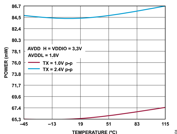
Figure 6. Power vs. Temperature, AVDD_H = 3.3 V, VDDIO = 3.3 V, AVDD_L = 1.8 V
