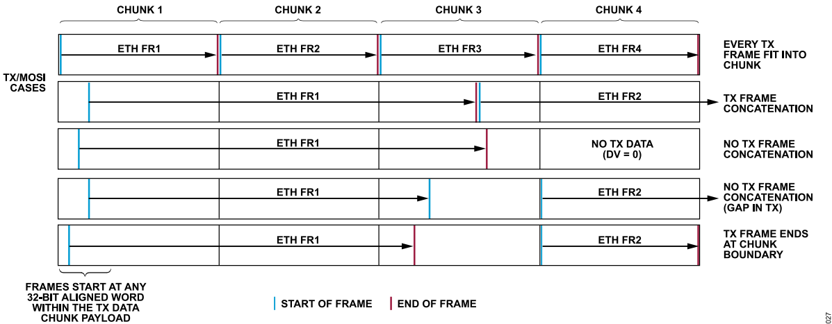
Figure 31. Transmit Data Chunk Cases
