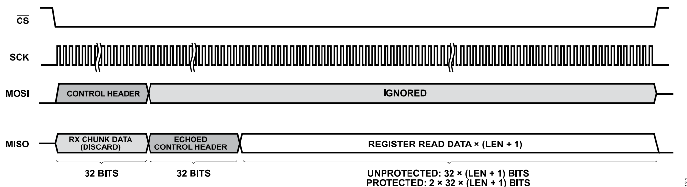
Figure 34. Control Read Transaction
