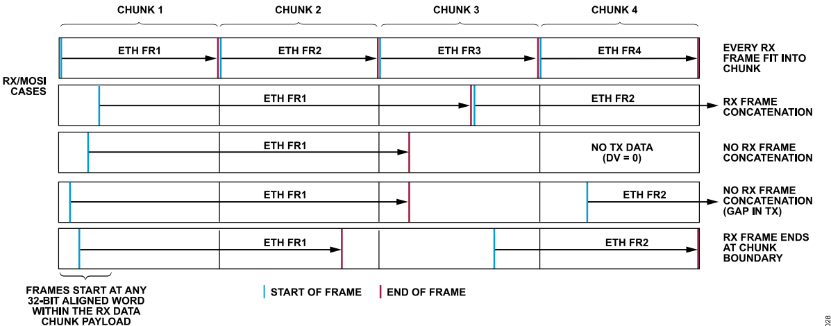
Figure 32. Receive Data Chunk Cases
