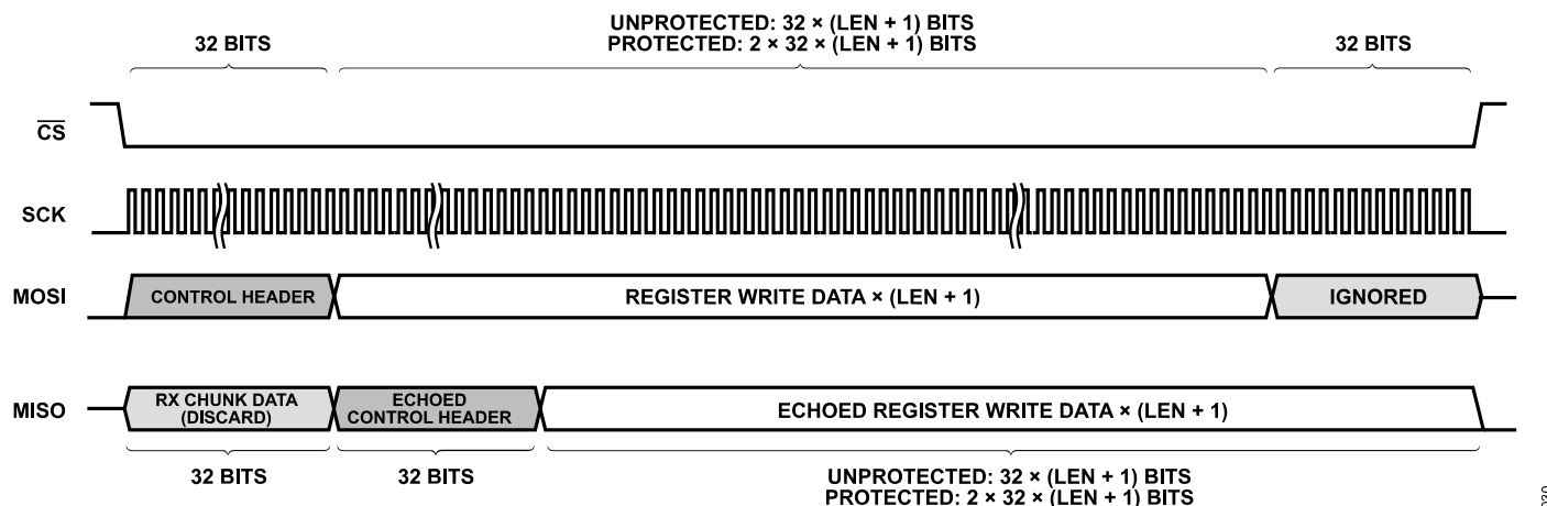
Figure 33. OPEN Alliance Control Transaction
