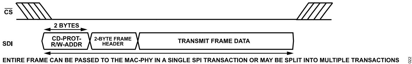
Figure 26. MAC Frame: Transmit
