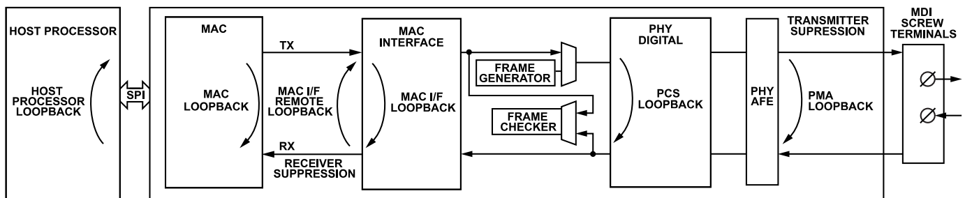
Figure 13. ADIN1111 Loopback Modes
