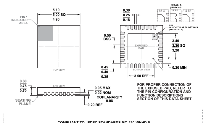
Figure 36. 32-Lead Lead Frame Chip Scale Package [LFCSP] 5 mm × 5 mm Body and 0.75 mm Package Height (CP-32-20) Dimensions shown in millimeters
