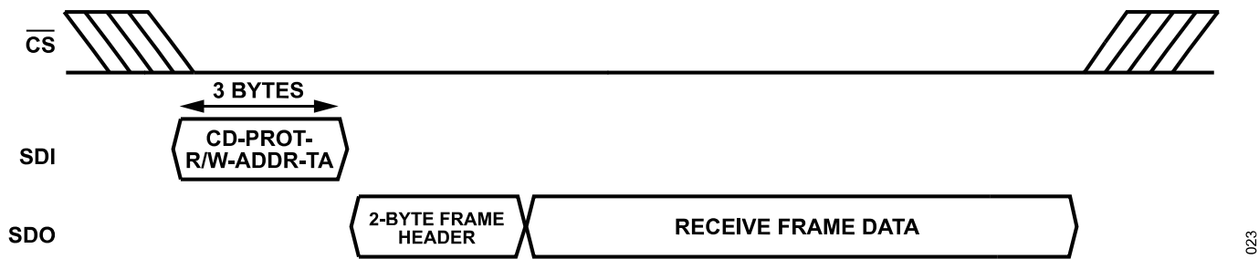
Figure 27. MAC Frame: Receive
