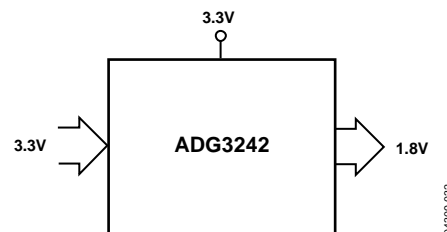
Figure 33. 3.3 V to 1.8 V Voltage Translation, \overline{SEL} = 0 V
