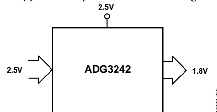
Figure 31. 2.5 V to 1.8 V Voltage Translation, \overline{SEL} = 2.5 V _{CC}
