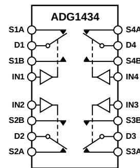
Figure 2. ADG1434 TSSOP
