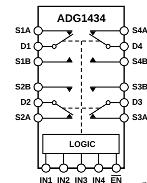
Figure 3. ADG1434 LFCSP
