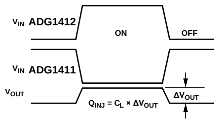
Figure 32. Charge Injection
