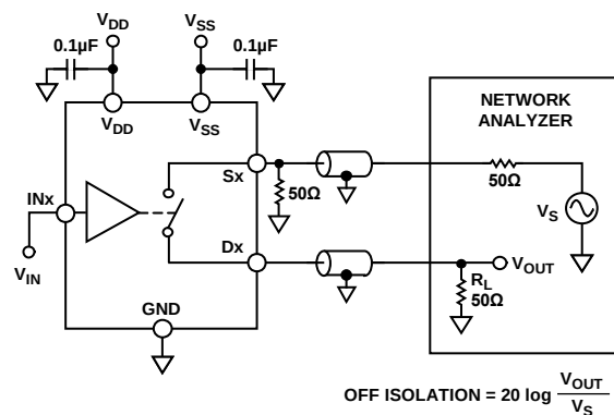
Figure 26. Off Isolation
