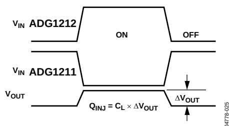
Figure 25. Charge Injection
