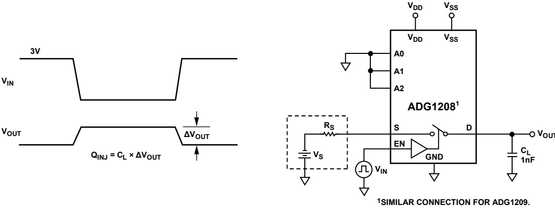
Figure 37. Charge Injection
