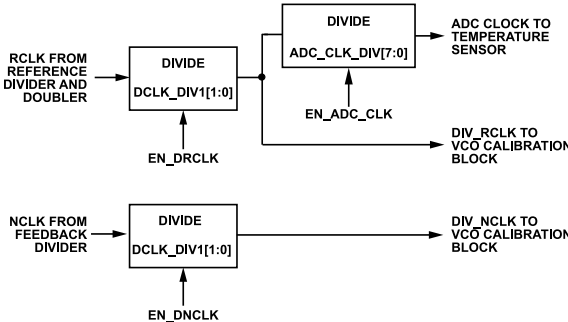
Figure 57. VCO Calibration Dividers
