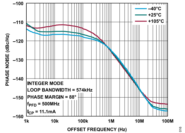
Figure 16. Closed-Loop Phase Noise vs. Offset Frequency at RFOUT = 20 GHz VCO Frequency Across Temperatures
