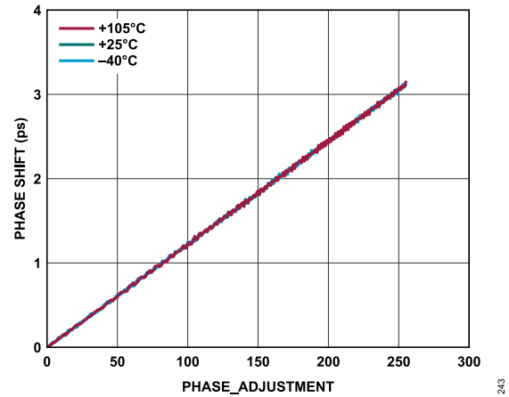
Figure 40. Phase Shift vs. PHASE\_ADJUSTMENT for Various Temperatures
