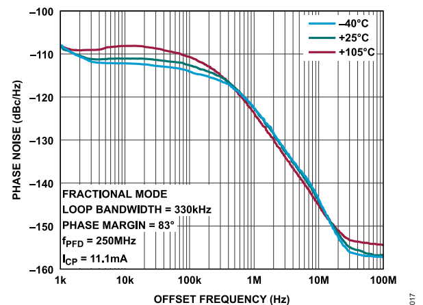
Figure 17. Closed-Loop Phase Noise vs. Offset Frequency at 19.9 GHz VCO Frequency Across Temperatures
