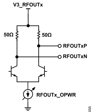
Figure 60. Simplified RF Output Buffer Schematic
