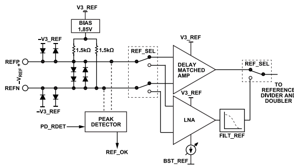
Figure 46. Reference Input Stage
