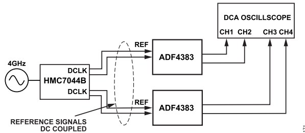
Figure 74. EZSync Configuration
