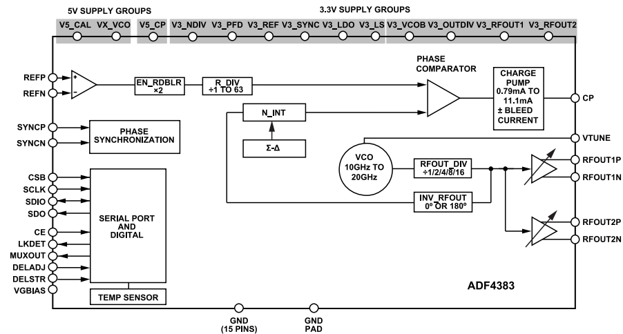
Figure 45. PLL Loop Diagram
