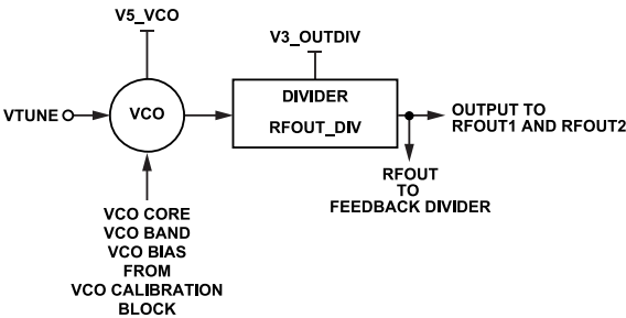
Figure 56. VCO and Clock Output Divider
