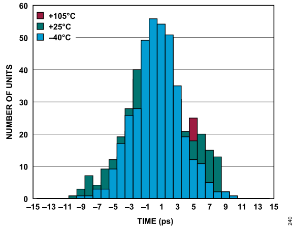
Figure 37. Normalized Propagation Delay ( t_{PD} ) Histogram
