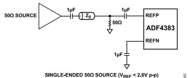
Figure 63. Single-Ended 50 \Omega Source ( V_{\text{REF}} < 2.6 \text{ V p-p} )
