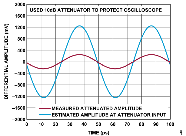
Figure 41. Differential Amplitude vs. Time at RFOUT = 20\text{ GHz}
