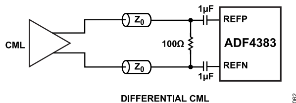
Figure 68. Differential CML
