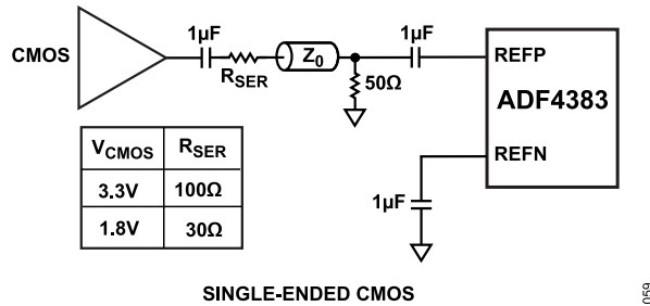
Figure 65. Single-Ended CMOS (R SER Is the Series Resistance.)
