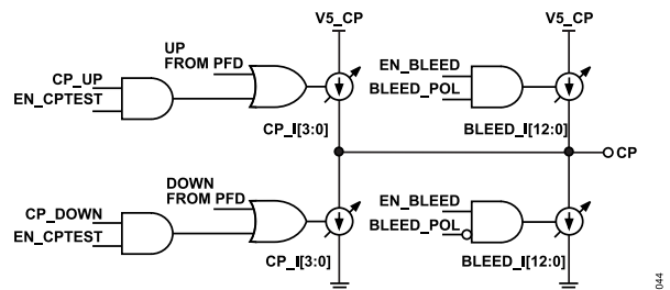
Figure 48. Simplified Charge Pump Schematic
