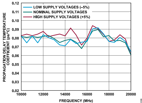
Figure 38. Propagation Delay Temperature Coefficient vs. Frequency
