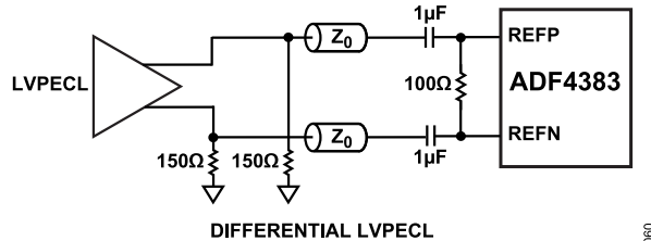
Figure 66. Differential, Low Voltage, Positive Emitter-Coupled Logic (LVPECL)
