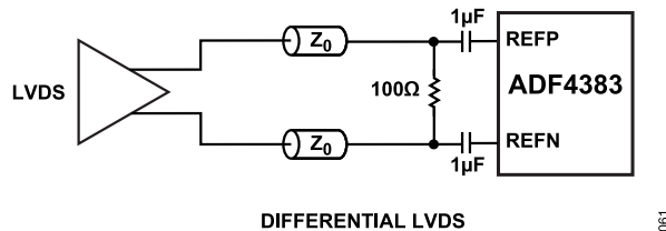
Figure 67. Differential LVDS
