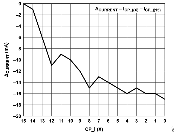
Figure 44. 5 V Delta Supply Current ( \Delta_{CURRENT} ) at Various CP_I Settings
