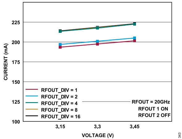
Figure 43. 3.3 V Supply Group 2 Current at Various Power Supply Voltages and RFOUT_DIV Settings
