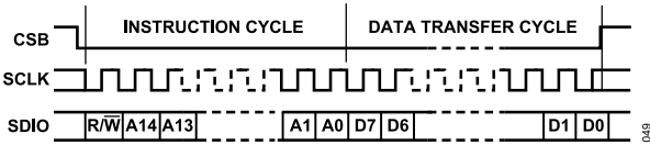
Figure 54. Serial Interface, MSB First (LSB_FIRST = 0)
