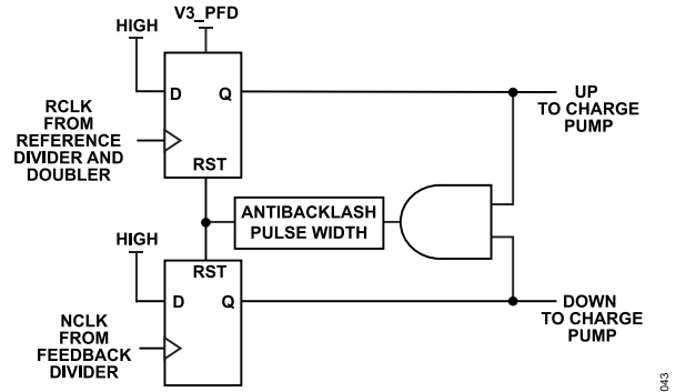
Figure 47. Simplified PFD Schematic
