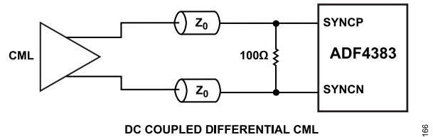
Figure 69. DC-Coupled Differential CML (Set SYNC_SEL = 0)
