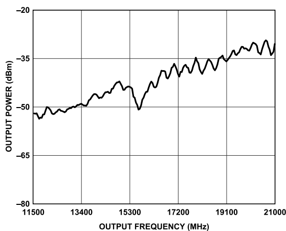
Figure 44. Output Power when Buffer Powered Down (PD_RFOUTx = 1) vs. Output Frequency
