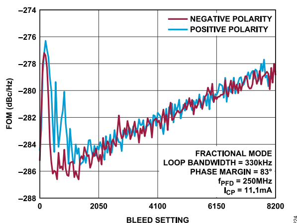
Figure 24. FOM, L_{1/f} Fractional Mode vs. Bleed Setting, f_{PFD} = 250 MHz, R_{FOUT} = 20.001 GHz
