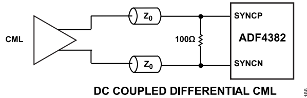
Figure 74. DC-Coupled Differential CML (Set SYNC_SEL = 0)
