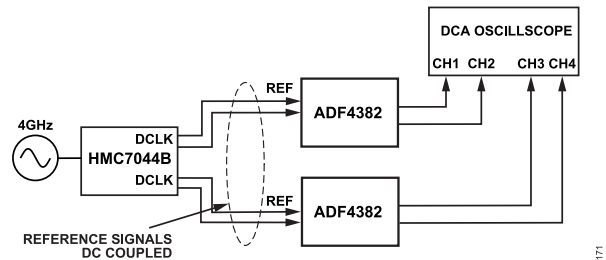
Figure 79. EZSync Configuration
