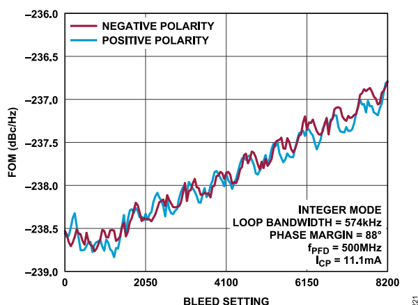
Figure 21. FOM, L_{NORM} Integer Mode vs. Bleed Setting, f_{PFD} = 500 MHz, R_{FOUT} = 20 GHz
