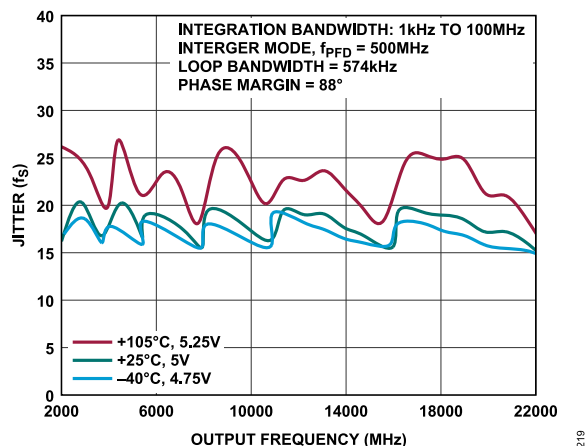
Figure 19. 1 kHz to 100 MHz Integrated Jitter in Integer Mode, f_{PFD} = 500 MHz
