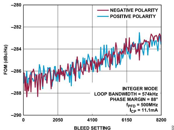
Figure 22. FOM, L_{1/f} Integer Mode vs. Bleed Setting, f_{PFD} = 500 MHz, R_{FOUT} = 20 GHz
