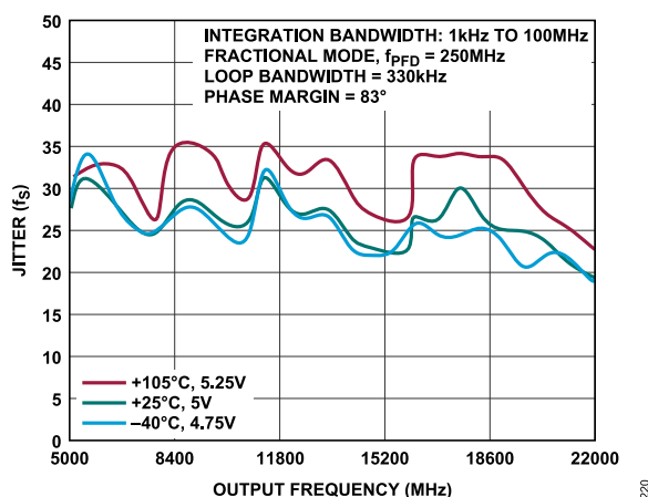
Figure 20. 1 kHz to 100 MHz Integrated Jitter in Fractional Mode, f_{PFD} = 250 MHz
