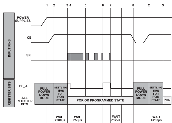
Figure 67. Power-Up and Initialization
