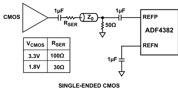
Figure 70. Single-Ended CMOS ( R_{SER} Is the Series Resistance.)
