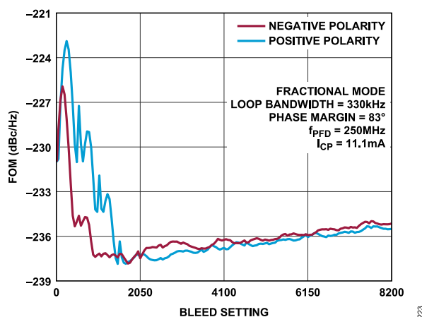
Figure 23. FOM, L_{NORM} Fractional Mode vs. Bleed Setting, f_{PFD} = 250 MHz, R_{FOUT} = 20.001 GHz
