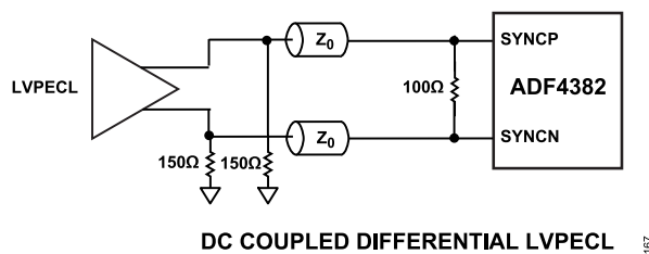
Figure 75. DC-Coupled Differential LVPECL (Set SYNC_SEL = 0)
