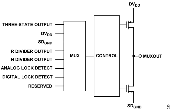
Figure 23. MUXOUT Schematic
