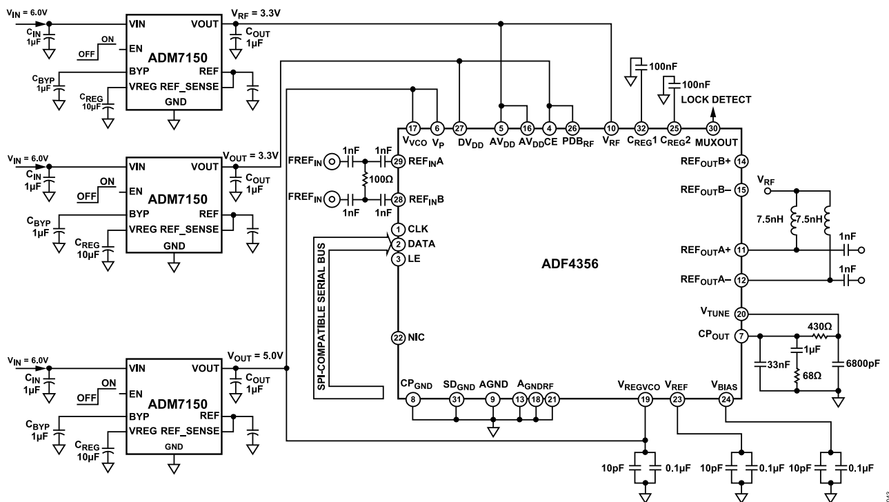
Figure 43. Power Supplies
