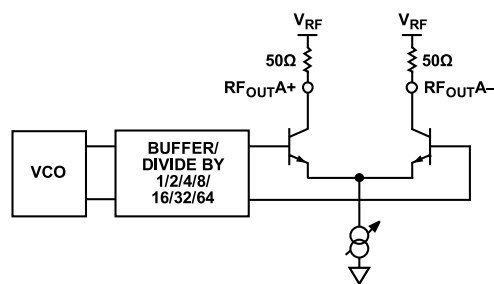
Figure 25. Output Stage
