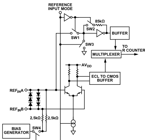
Figure 20. Reference Input Stage, Differential Mode
