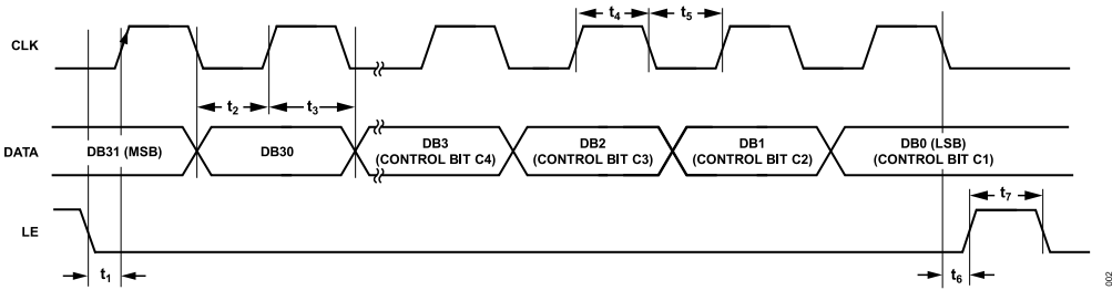
Figure 2. Write Timing Diagram
