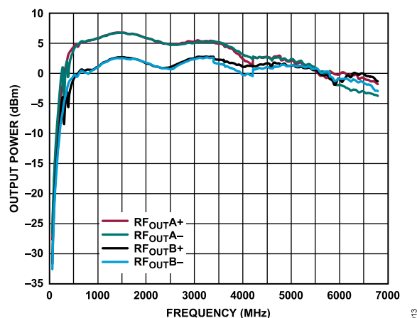
Figure 13. RF_{OUTA+}/RF_{OUTA-} Power vs. RF_{OUTB+}/RF_{OUTB-} Power (7.4 nH Inductors, 10 pF AC Coupling Capacitors, Board Measurement)
