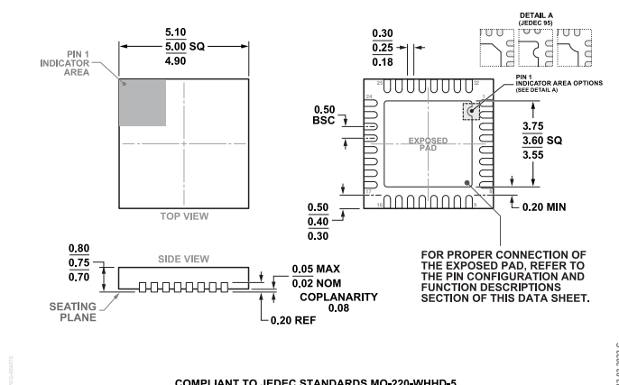
Figure 45. 32-Lead Lead Frame Chip Scale Package [LFCSP] 5 mm x 5 mm Body and 0.75 mm Package Height (CP-32-12) Dimensions shown in millimeters
