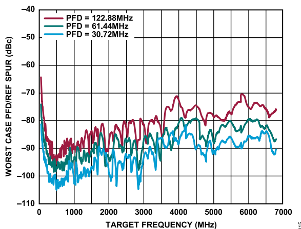
Figure 15. PFD Spur Amplitude vs. RF_{OUTA+}/RF_{OUTA-} Output Frequency, PFD = 30.72 MHz, PFD = 61.44 MHz, PFD = 122.88 MHz, Loop Filter = 40 kHz
