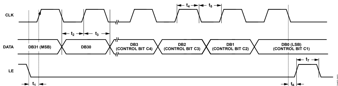
Figure 2. Timing Diagram
