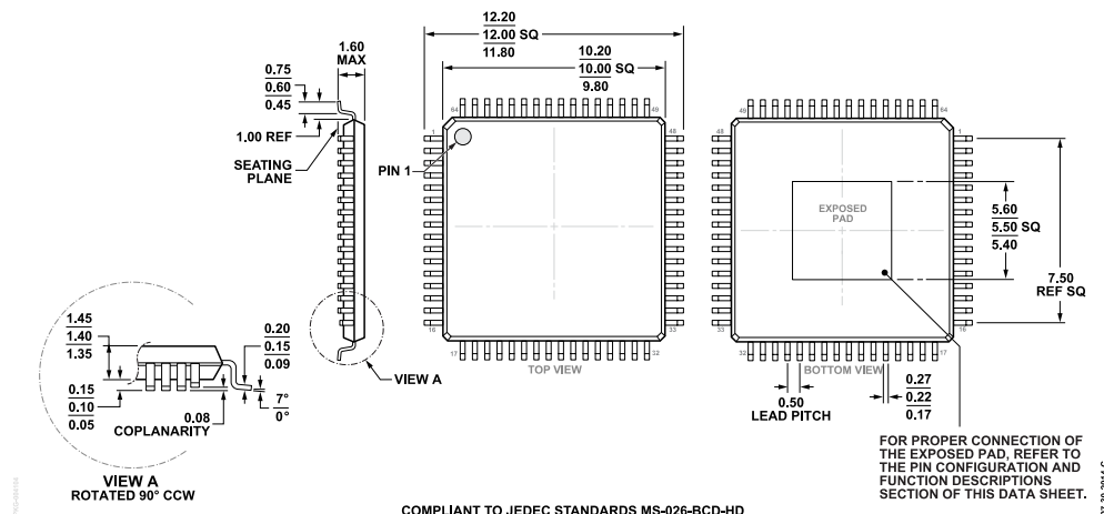
Figure 114. 64-Lead Low Profile Quad Flat Package, Exposed Pad [LQFP_EP] (SW-64-2)
