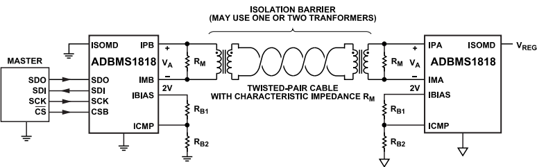
Figure 103. isoSPI Circuit
