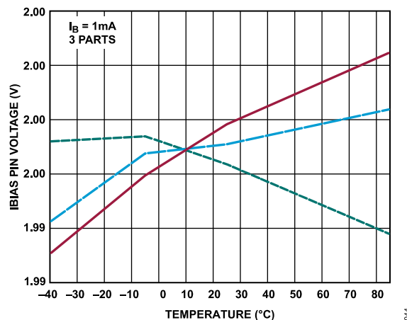
Figure 44. IBIAS Pin Voltage vs. Temperature
