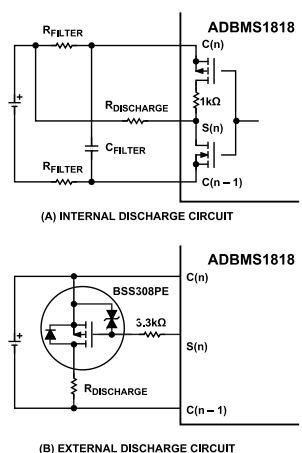
Figure 99. Internal/External Discharge Circuits
