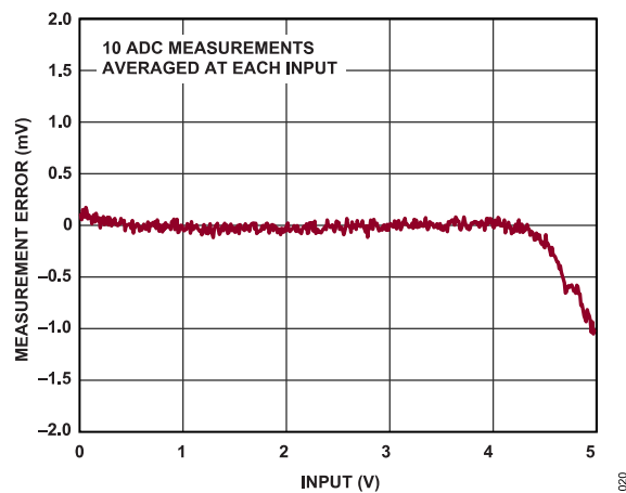
Figure 20. Measurement Error vs. Input, Normal Mode
