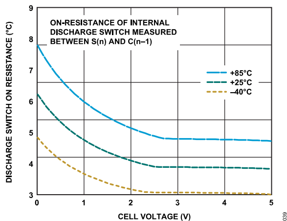
Figure 39. Discharge Switch On Resistance vs. Cell Voltage
