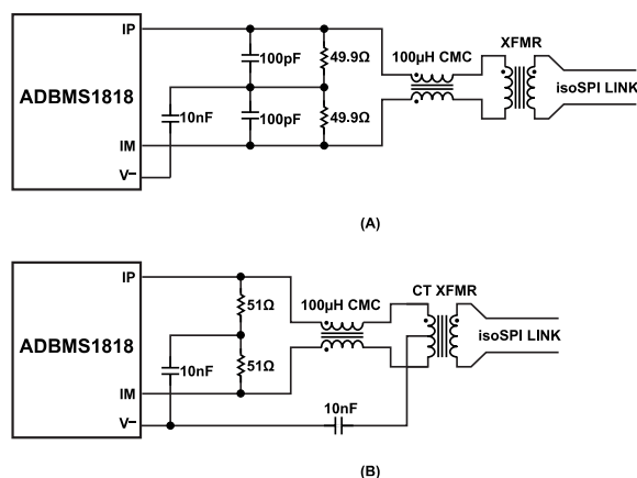
Figure 104. Daisy Chain Interface Components
