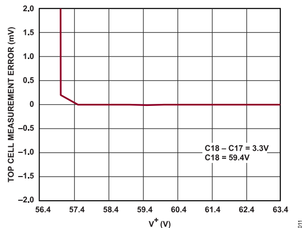
Figure 11. Top Cell Measurement Error vs. V^*
