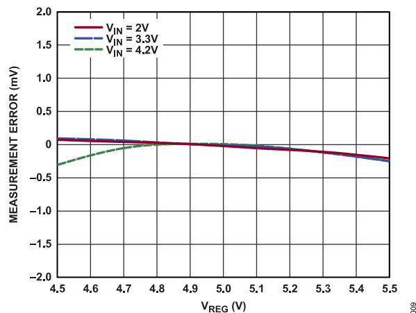
Figure 9. Measurement Error vs. V_{REG}
