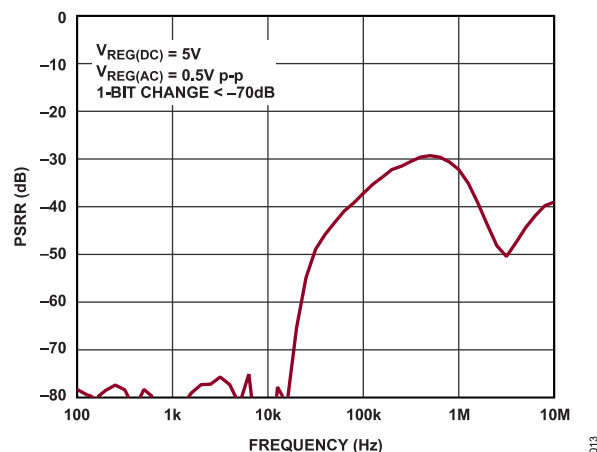
Figure 13. Measurement Error Due to a V_{REG} AC Disturbance
