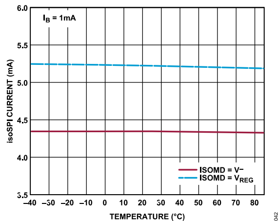
Figure 42. isoSPI Current (Ready) vs. Temperature
