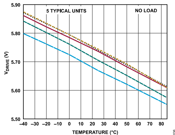
Figure 36. V_{DRIVE} vs. Temperature
