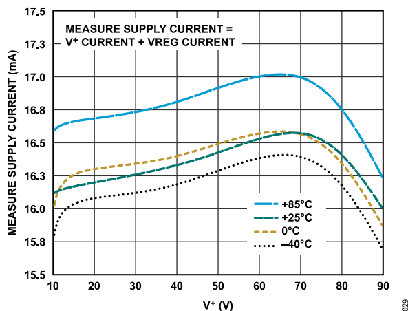
Figure 29. Measure Supply Current vs. V +
