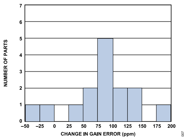
Figure 7. Measurement Error Due to IR Reflow
