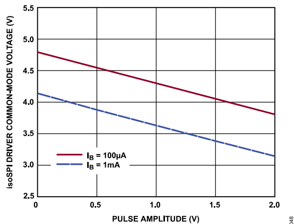
Figure 48. isoSPI Driver Common-Mode Voltage (Port A and Port B) vs. Pulse Amplitude
