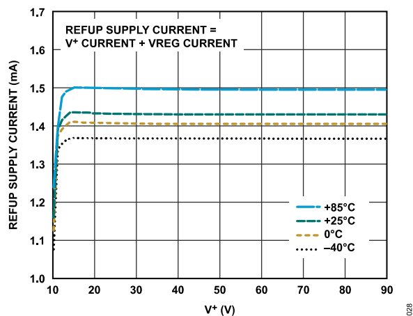
Figure 28. REFUP Supply Current vs. V +
