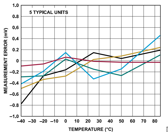
Figure 19. Measurement Error vs. Temperature
