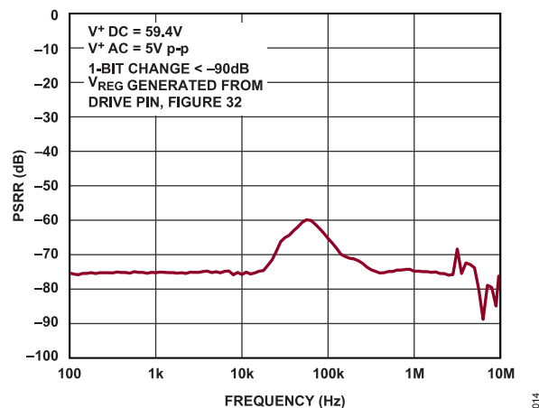
Figure 14. Measurement Error Due to a V^* AC Disturbance (PSRR is Power Supply Rejection Ratio)
