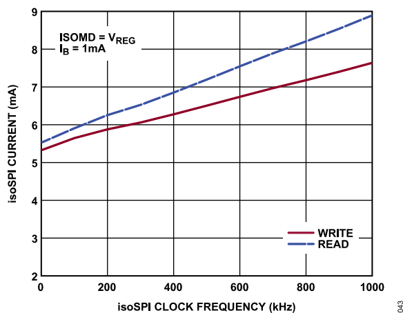
Figure 43. isoSPI Current (Active) vs. isoSPI Clock Frequency
