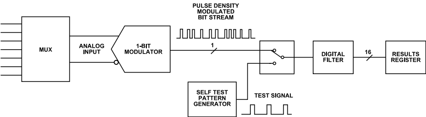
Figure 62. Operation of ADBMS1818 ADC Self Test
