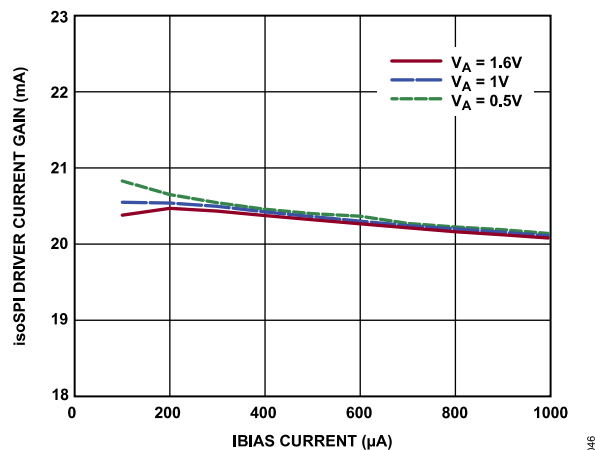
Figure 46. isoSPI Driver Current Gain (Port A and Port B) vs. IBIAS Current
