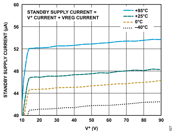
Figure 27. Standby Supply Current vs. V +
