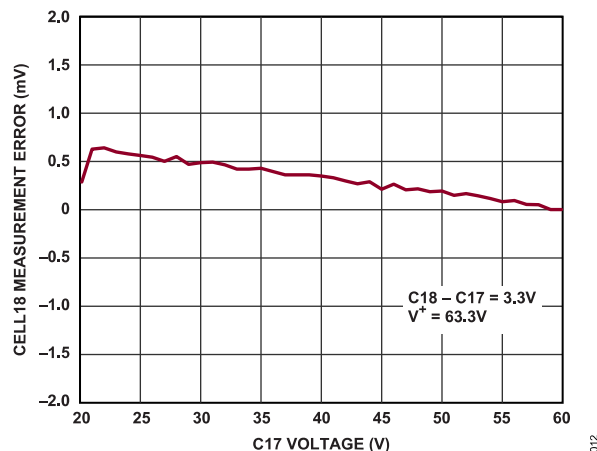
Figure 12. Measurement Error vs. Common-Mode Voltage
