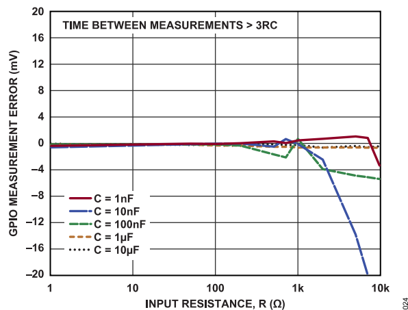
Figure 24. GPIO Measurement Error vs. Input RC Values
