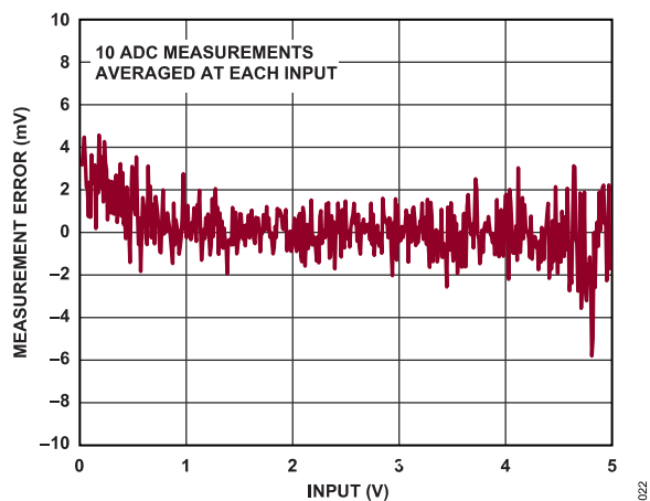
Figure 22. Measurement Error vs. Input, Fast Mode
