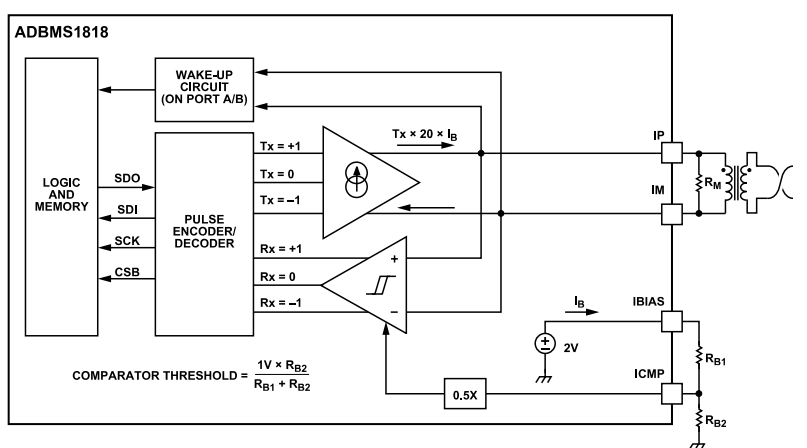
Figure 78. isoSPI Interface
