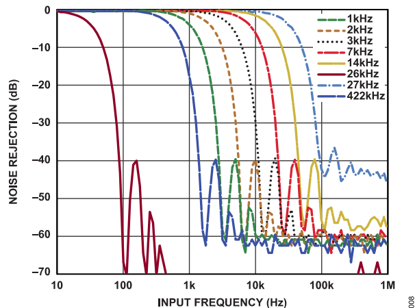
Figure 8. Noise Filter Response
