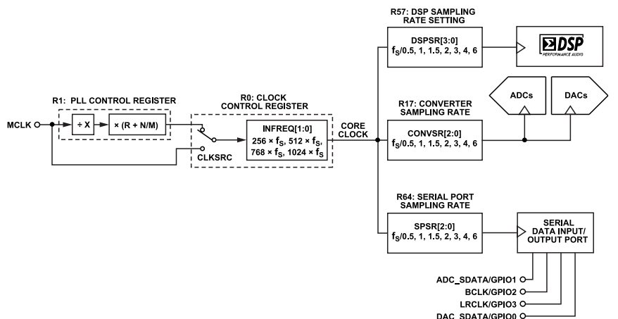
Figure 30. Clock Tree Diagram
