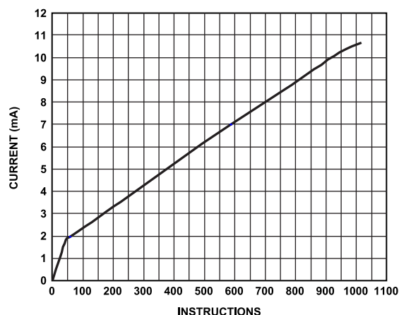
Figure 22. Typical DSP Current Draw
