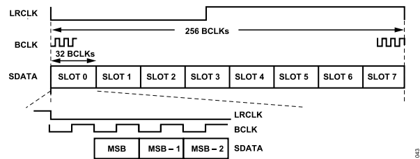
Figure 61. TDM 8 Mode
