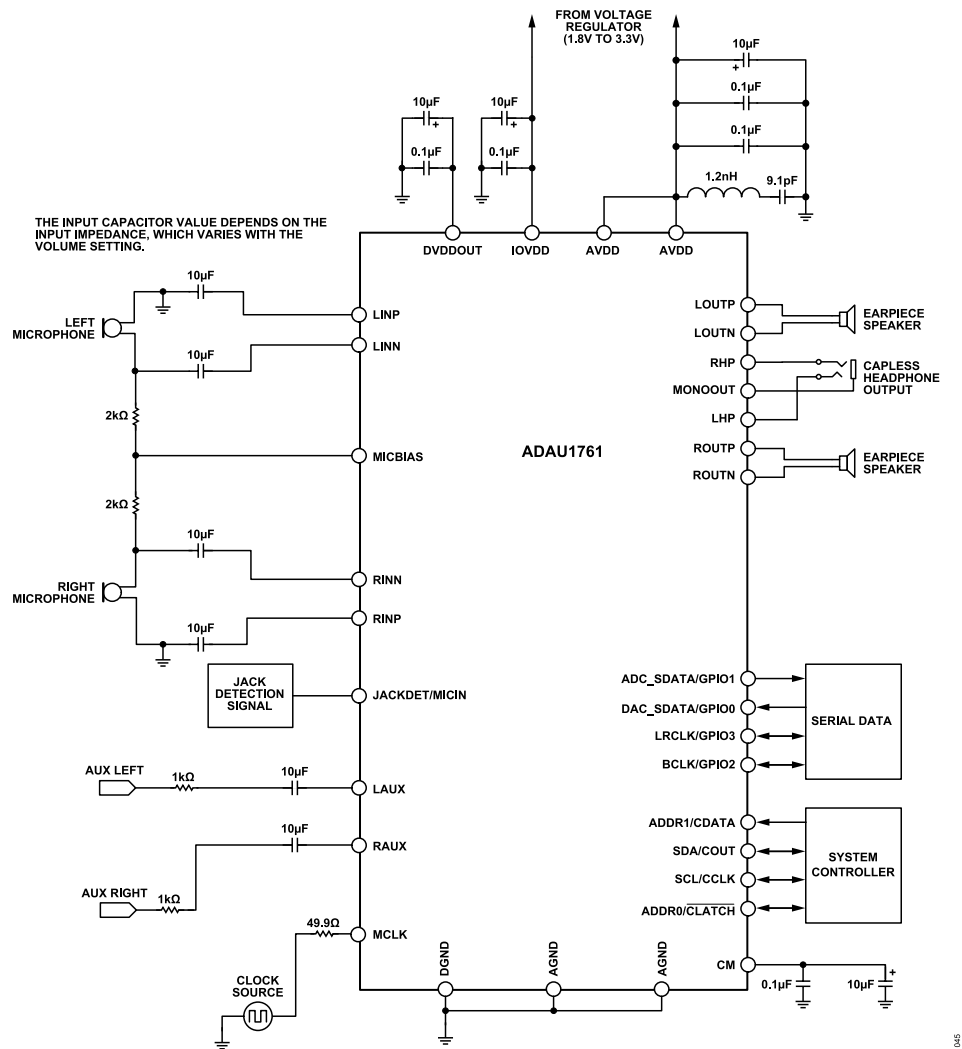
Figure 26. System Block Diagram
