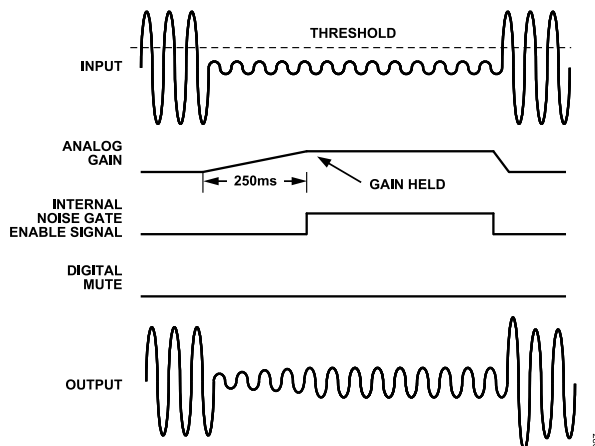
Figure 40. Noise Gate Mode 0 (PGA Gain Hold)
