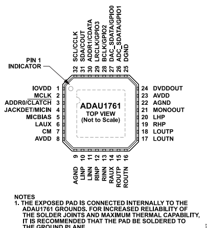
Figure 7. Pin Configuration
