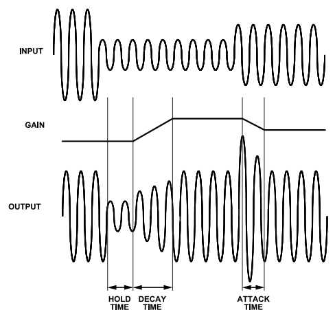
Figure 38. Basic ALC Operation
