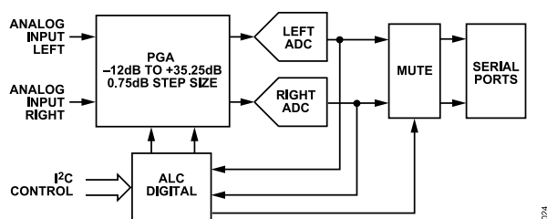
Figure 37. ALC Architecture
