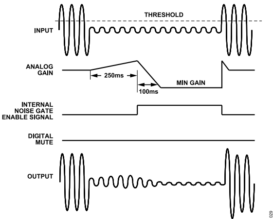
Figure 42. Noise Gate Mode 2 (Analog Fade)
