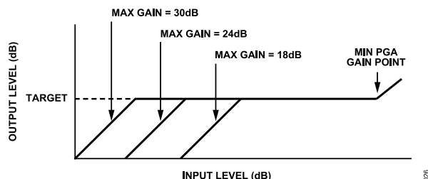
Figure 39. Effect of Varying the Maximum Gain Parameter
