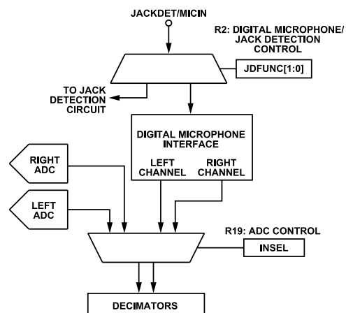
Figure 36. Digital Microphone Interface Block Diagram
