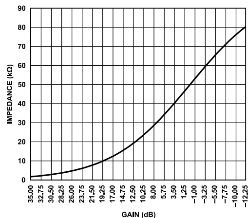
Figure 25. Input Impedance vs. Gain for Analog Inputs
