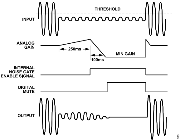
Figure 43. Noise Gate Mode 3 (Analog Fade/Digital Mute)
