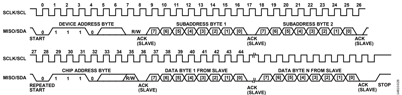
Figure 30. I²C Slave Burst Mode Read Operation (N Bytes)
