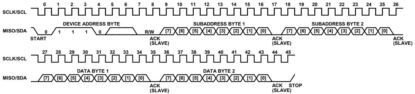
Figure 28. I²C Slave Single Word Write Operation (Two Bytes)
