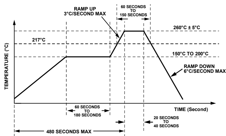
Figure 92. Soldering Profile
