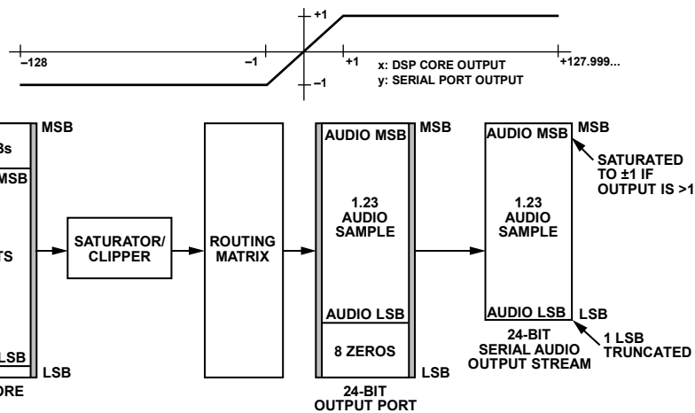
Figure 70. 24-Bit Serial Output Example
