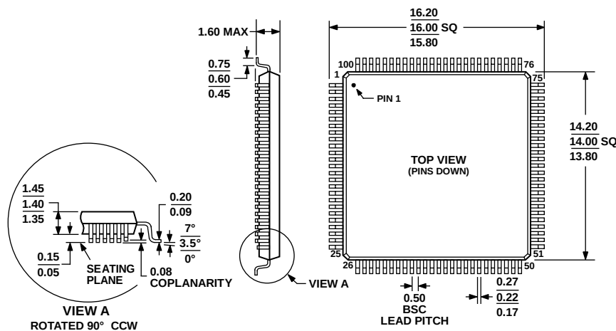
COMPLIANT TO JEDEC STANDARDS MS-026-BED Figure 68. 100-Lead Thin Quad Flat Package [LQFP] (ST-100-1) Dimensions shown in millimeters
