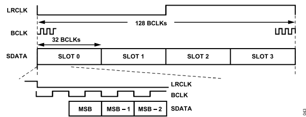
Figure 60. TDM 4 Mode
