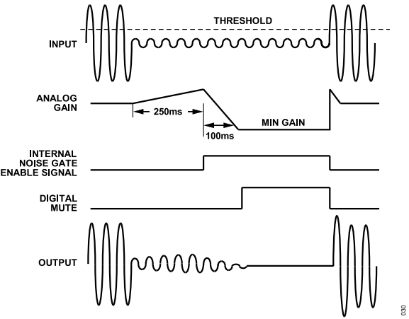
Figure 42. Noise Gate Mode 3 (Analog Fade/Digital Mute)
