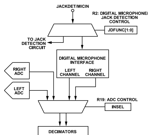
Figure 35. Digital Microphone Interface Block Diagram
