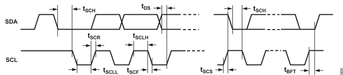
Figure 5. I 2 C Port Timing
