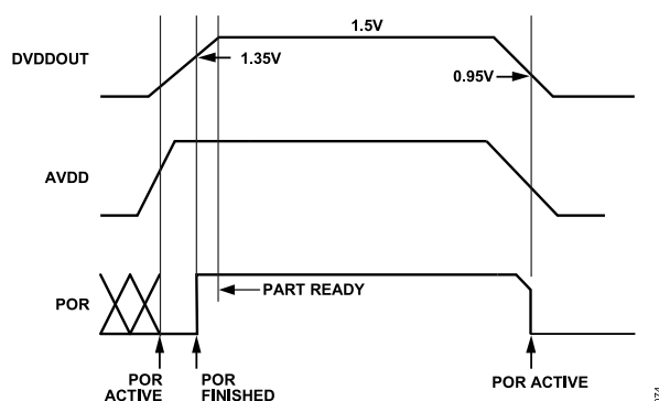
Figure 28. Power-On Reset Sequence
