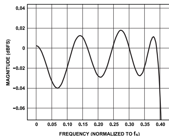
Figure 18. ADC Decimation Filter Pass-Band Ripple, 128× Oversampling, Double-Rate Mode, Normalized to f_s
