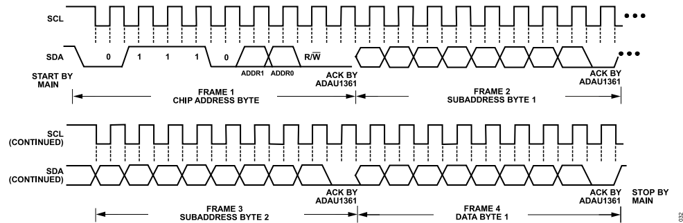
Figure 48. I 2 C Write to ADAU1361 Clocking
