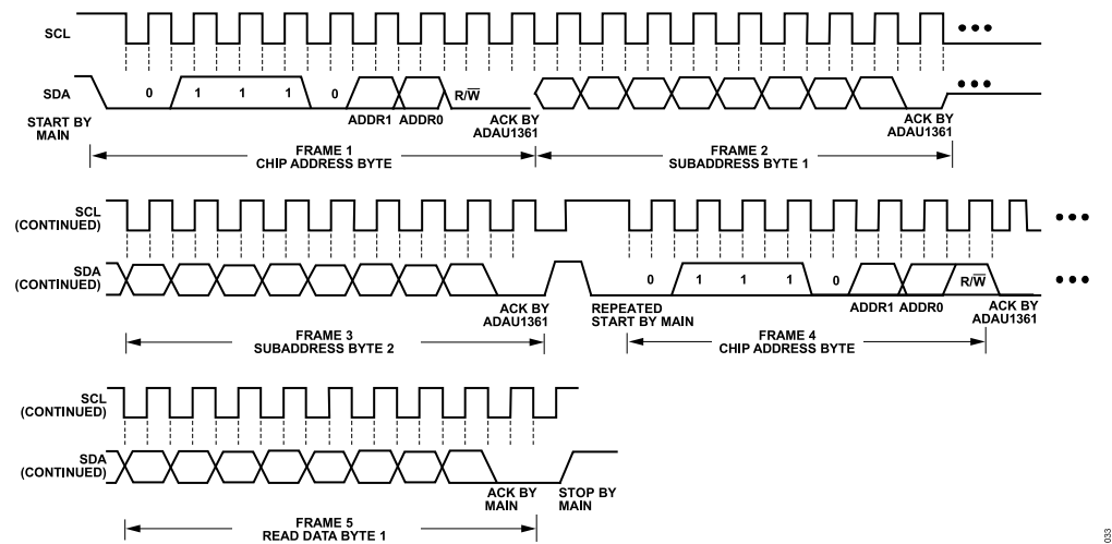
Figure 49. I 2 C Read from ADAU1361 Clocking
