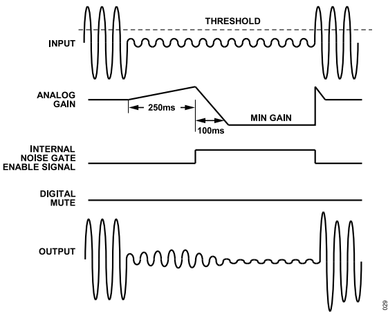
Figure 41. Noise Gate Mode 2 (Analog Fade)
