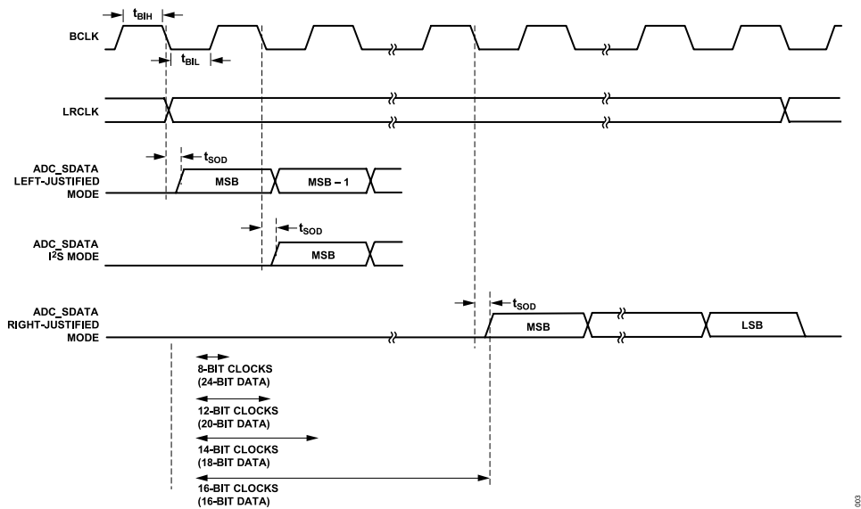
Figure 3. Serial Output Port Timing
