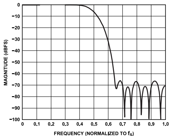
Figure 21. DAC Interpolation Filter, 128x Oversampling, Double-Rate Mode, Normalized to f_s
