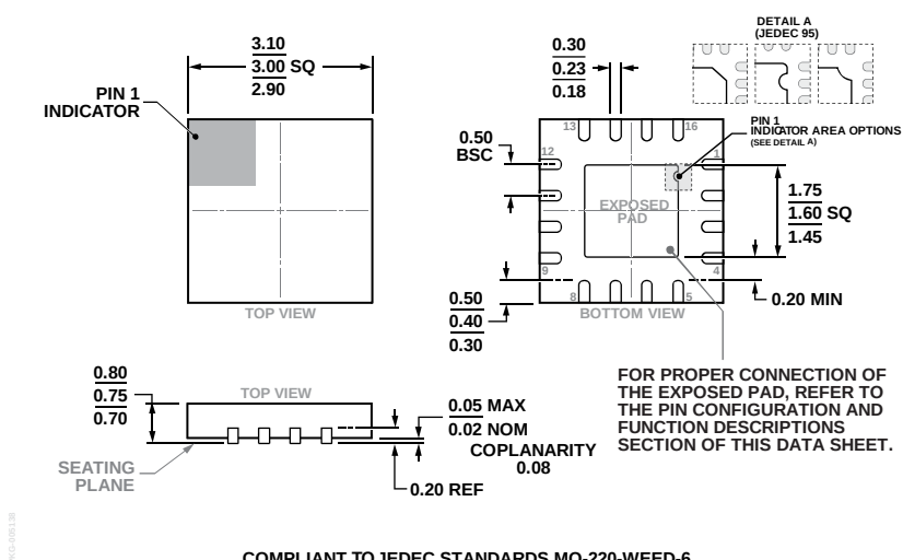
Figure 46. 16-Lead Lead Frame Chip Scale Package [LFCSP] 3 mm × 3 mm Body and 0.75 mm Package Height (CP-16-22)
